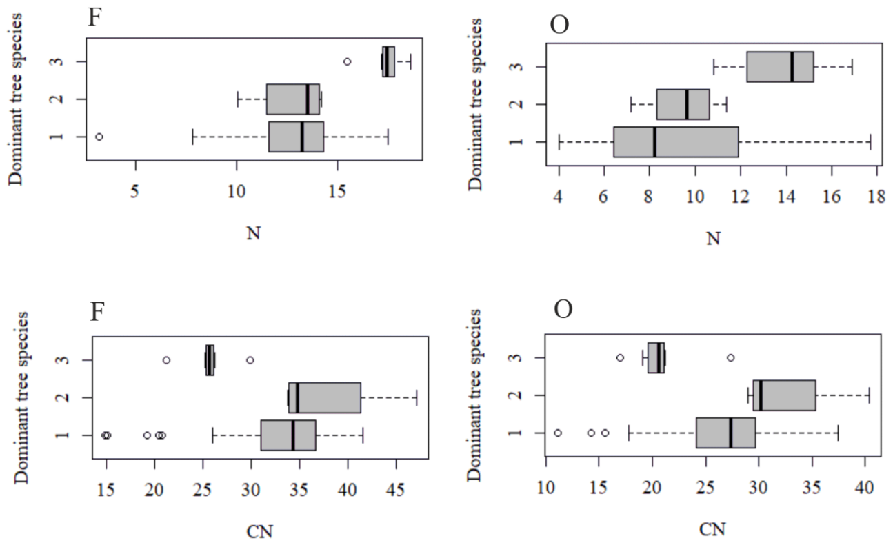
Figure 4. Soil total N content (upper panel) and soil C:N ratio (lower panel) of the research plots (based on dominant tree species) in soil horizons F and O. Species 1 = pine, 2 = spruce and 3 = birch.
