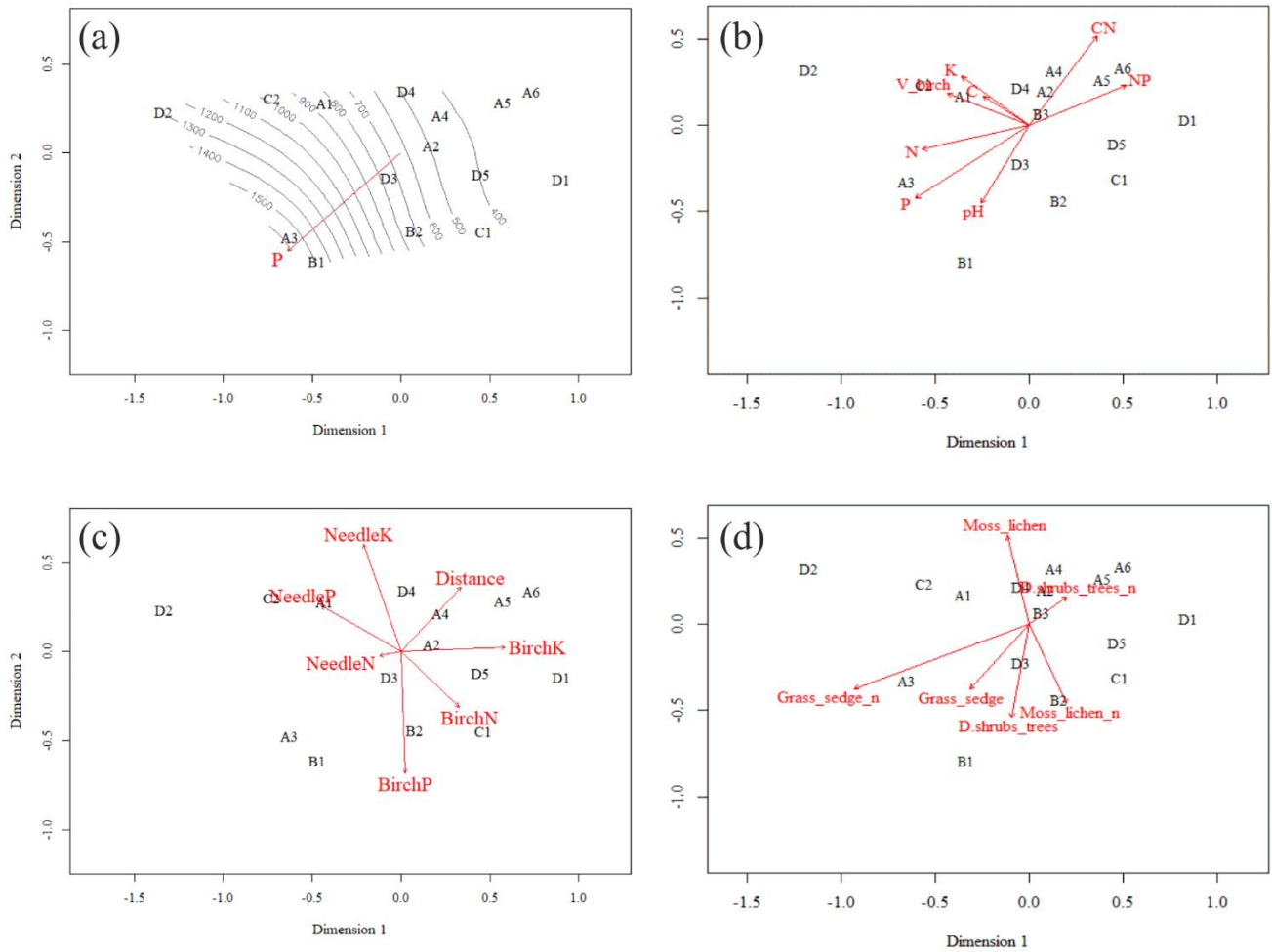
5 Figure 7: Ordination pattern with smooth surface fit and linear vector fit of soil phosphorus (P) in the O layer (a), linear vector fits of soil element contents in the O layer (b), linear vector fits of foliar data as well as plot distance from Sokli phosphate ore (c), and linear vector fits of number of species in different layers of understory (d). Moss_lichen includes moss and lichen species, Grass_sedge includes forb, grass, and sedge species and D.shrubs_trees includes dwarf shrubs and tree seedlings. In (a) and (c) plots D4 and B3 were located on top of each other and only D4 is shown.
