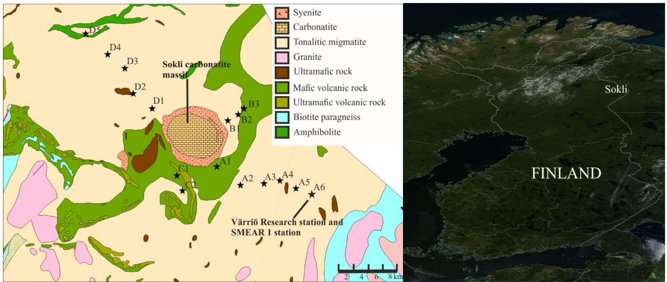
Figure 1: Left: Geological map of the research area. Plots are marked with black stars. The easternmost plot is located at the SMEAR1 station. (Source: Hakku Service, https://hakku.gtk.fi/en/locations/search .), Right: Satellite image showing the study location (source: NASA).
