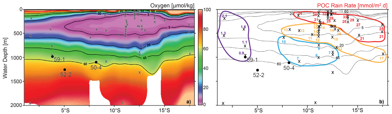
Figure 2: a) Depth vs latitude profile of the dissolved oxygen concentrations measured during the M77 Leg & 2 expeditions (red line in Figure 1, b show the position of this profile; CTD data compilation after Schönfeld et al., 2015); together with the location of the surface samples (x), the sediment cores (circles and core names), b) particulate organic carbon rain rates (RRPOC) taken from Dale et al. (2015) otherwise calculated following Martin et al. (1987). Rain rates are grouped indicating different values ( < 5 , 5-10, 10-20 and > 20 mmol/m 2 d), see text for details. Contour lines are the same as in a.
