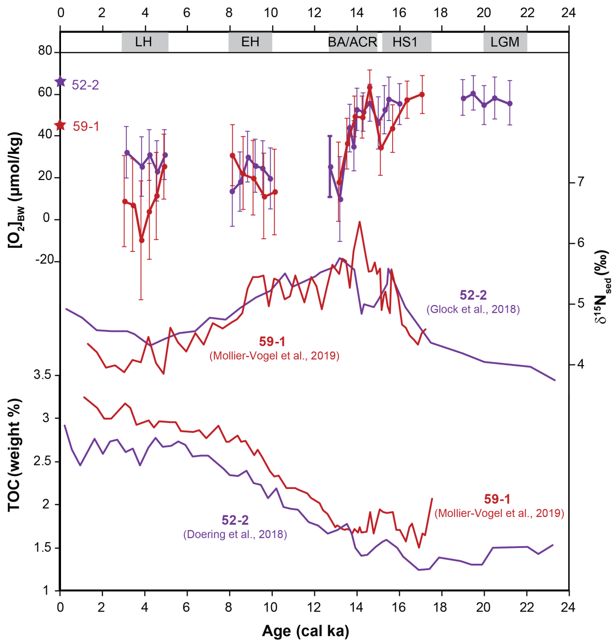
Figure 7: Comparison of [O_2]_{BW} estimated concentrations with bulk sedimentary \delta^{15}N and TOC (w.%) from the same cores (data is available for cores M77/2-59-1 and M77/2-52-2).
