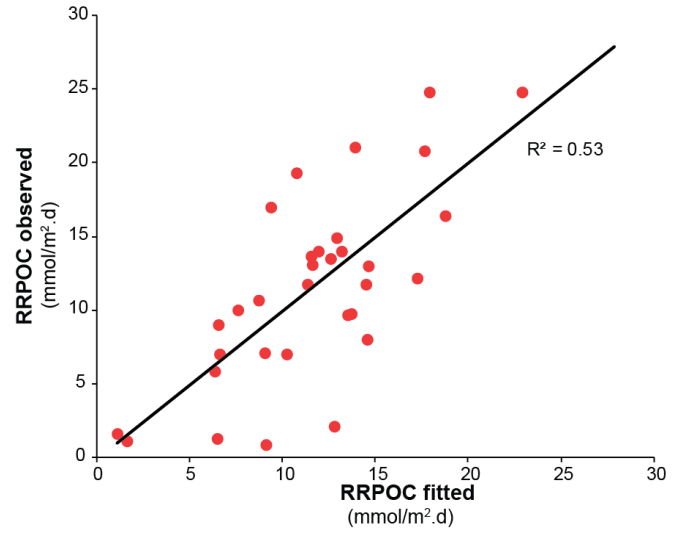
5 Figure 5: Graphs showing the regression results applied to the living benthic foraminifera dataset for bottom water oxygen ([O 2 ] BW ) and POC rain rates (RRPOC).
