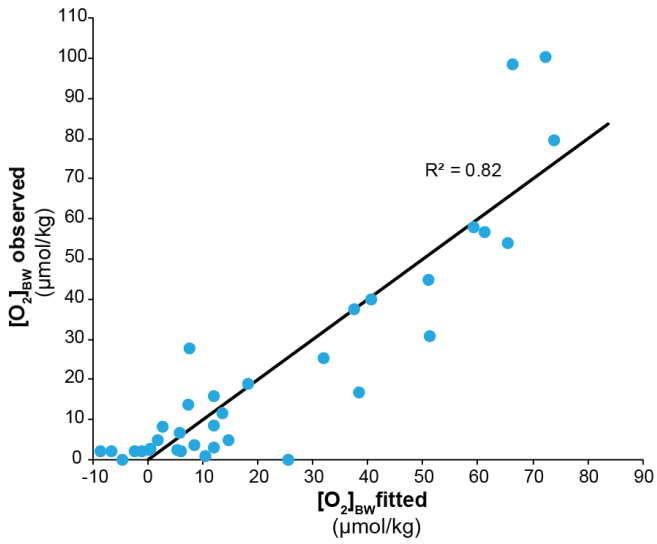
5 Figure 5: Graphs showing the regression results applied to the living benthic foraminifera dataset for bottom water oxygen ([O 2 ] BW ) and POC rain rates (RRPOC).
