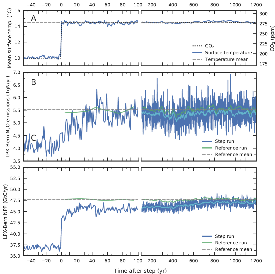
Figure 11: Response to a step-like change in (A) environmental conditions for globally averaged terrestrial (B) \text{-N}_2\text{O} emissions and (C) NPP. Atmospheric \text{CO}_2 (dotted line in (A)) and climate is prescribed to suddenly change from Last Glacial Maximum conditions to late Holocene conditions in a sensitivity simulation with LPX-Bern( v1.4 v1.4N ) (“step run”, blue lines). Annual values for the step run are shown in dark blue and smoothed (31-yr average) values in light blue for the step run and in dark green for a corresponding reference run. The dashed horizontal lines represent averages from the reference run over the model period 0 to 1200 years. Surface air temperature in (A) represents the average over the model’s land area. Note the change in the time axis scaling at year 100.
