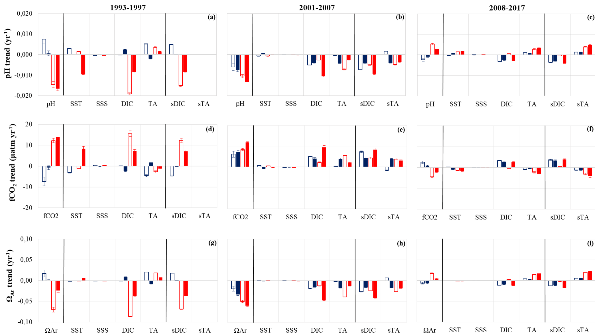
Figure 5. Decomposition of the trends in surface pH (a-c), f\text{CO}_2 (d-f) and \Omega_{\text{Ar}} (g-i) according to equation (2). The effect of the changes in SSS, SST, DIC, TA and the normalized part (sDIC and sTA) is shown for the three periods: 1993-1997 (left column), 2001-2007 (middle column) and 2008-2017 (right column). Color coding is the same as in Figure 4. Here, DIC (or TA) represent the total carbon (or total alkalinity) part, whereas sDIC (or sTA) is the part of DIC (or TA) driver not related to salinity (see explanations for Eq. 2).
