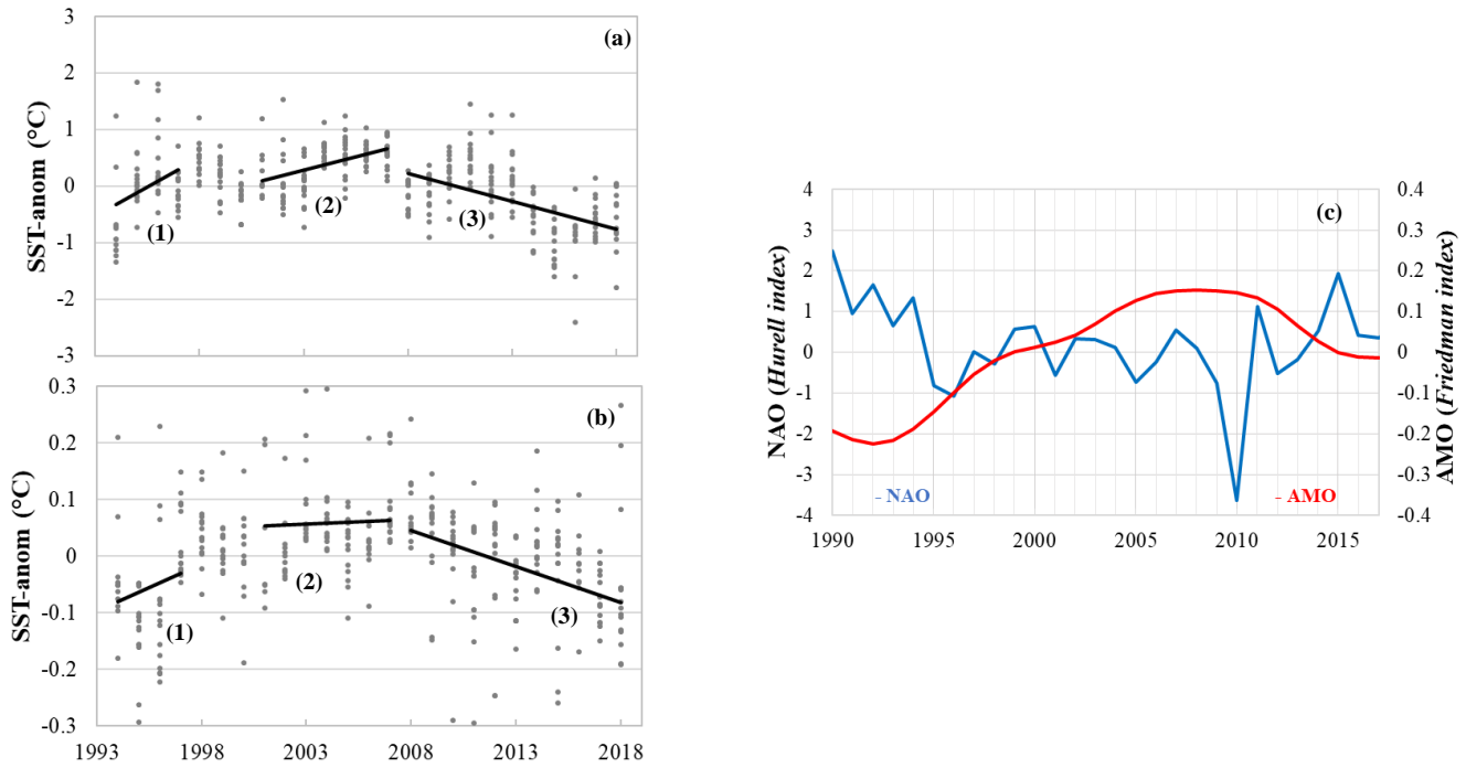
Figure 3. SST (a) and SSS (b) anomalies for winter (jan-feb) along Suratlant track (north of 50°N), based on the Binned products constructed by Reverdin et al. (2018a) and updated data to 2018, available at https://doi.org/10.6096/SSS-BIN-NASG , last access 25/03/2020). The mean trends for each period selected for the carbonate data analysis (when available) are represented in black lines (1: 1993-1997, 2: 2001-2007, 3: 2008-2017). The NAO index (in blue, Hurrell data available at https://climatedataguide.ucar.edu/climate-data/hurrell-north-atlantic-oscillation-nao-index-station-based , last access 30/09/2019) and AMO index (in red, Friedman ERSST V5 data available at https://www.ncdc.noaa.gov/data-access/marineocean-data/extended-reconstructed-sea-surface-temperature-ersst-v5 , last access 20/11/2019) are represented (c).
