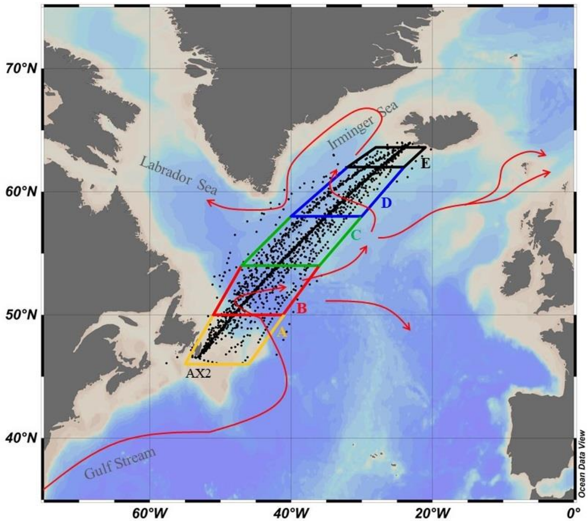
Figure 1. SURATLANT cruises track (in black, TA/DIC data over the period 1993-2017) with the five boxes [BOX A: 46°N-50°N (in yellow), Box B: 50°N-54°N (in red), Box C: 54°N-58°N (in green), Box D: 58°N-62°N (in blue), Box E: 62°N-64°N (in black)] and surface currents in the North Atlantic Subpolar Gyre (NASPG) circulation resulting from the Gulf Stream and the North Atlantic Current (in red).
