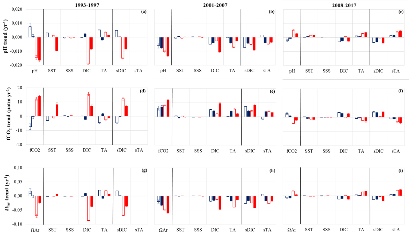
Figure 5. Decomposition of the trends in surface pH (a-c), f\text{CO}_2 (d-f) and \Omega_{\text{Ar}} (g-i) according to equation (2). The effect of the changes in SSS, SST, DIC, TA and the normalized part (sDIC and sTA) is shown for the three periods: 1993-1997 (left column), 2001-2007 (middle column) and 2008-2017 (right column). Color coding is the same as in Figure 4. Here, DIC (or TA) represent the total carbon (or total alkalinity) part, whereas sDIC (or sTA) is the part of DIC (or TA) driver not related to salinity (see explanations for Eq. 2).
