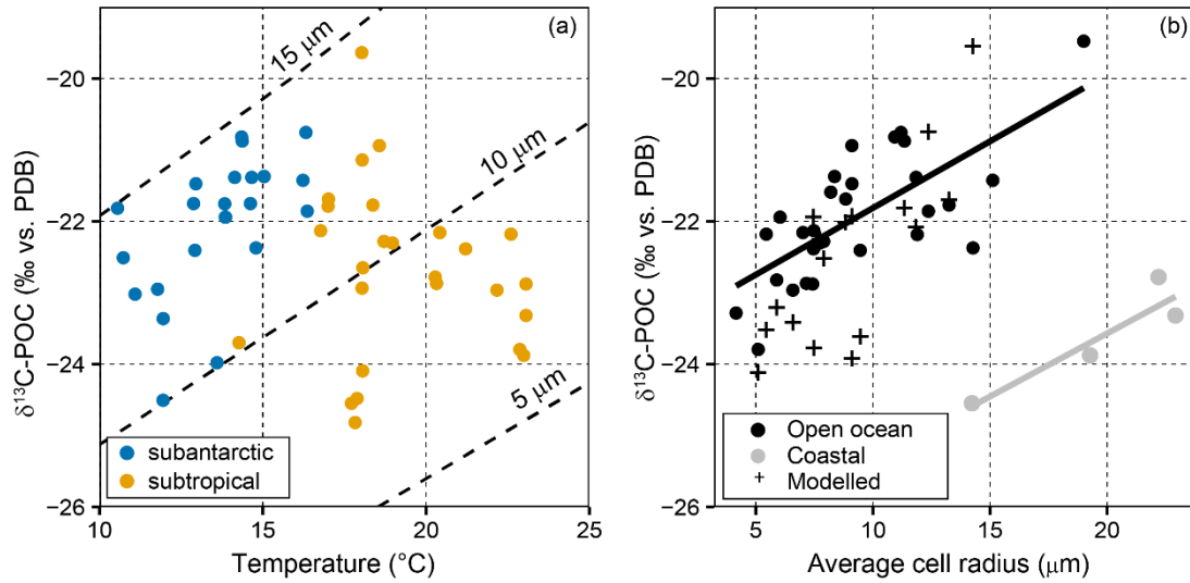
5 Figure 6. \delta^{13}\text{C}_{\text{POC}} variability and model predictions with temperature and cell size. (a) \delta^{13}\text{C}_{\text{POC}} versus temperature, with the modelled estimates for cell radii of 5, 10 and 15 \mu\text{m} . Blue circles = SASW, orange circles = subtropical waters. (b) \delta^{13}\text{C}_{\text{POC}} vs cell radius as derived from pigment data. Samples from the eastern and western margin are excluded from correlation estimates. Rio Plata: r=0.92 , df=2 , p=0.075 ; Open ocean: r=0.72 , df=30 , p<0.001 . Modelled \delta^{13}\text{C}_{\text{POC}} is estimated using measured temperature and cell size and an assumed constant cell growth rate of 1.1 \text{ d}^{-1} . Black crosses show modelled results. Average cell radius calculated from micro-plankton (25 \mu\text{m} ), nano-plankton (2.5 \mu\text{m} ) and pico-plankton (0.5 \mu\text{m} ). There are less data in (b) as we did not have corresponding cell size data for all of the \delta^{13}\text{C}_{\text{POC}} measurements.
