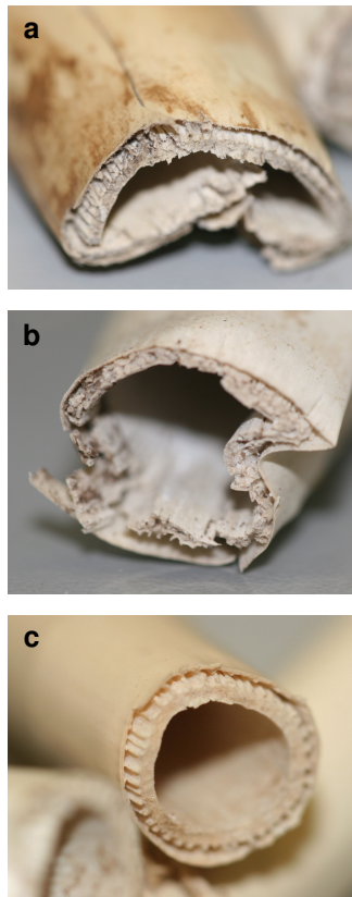
Figure 8. P. australis rhizomes after 75 days of anaerobic decomposition in the three peat substrates. (a): high-N substrate (detritus mud), (b): medium-N substrate ( c3 sedge-brown-moss peat ), and (c): low-N substrate ( Sphagnum peat).
