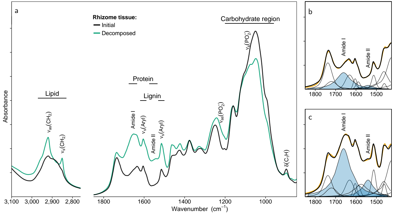
Figure 3. FTIR spectroscopic analysis of changes in rhizome c62 tissue chemical composition after decomposition in the medium-N soil. (a): FTIR absorption spectra. c63 (b & c): Peak fitting of the FTIR spectra of the initial and decomposed c64 rhizomes. c65 Plotted bands in blue denote the amide I and amide II bands of proteins.
