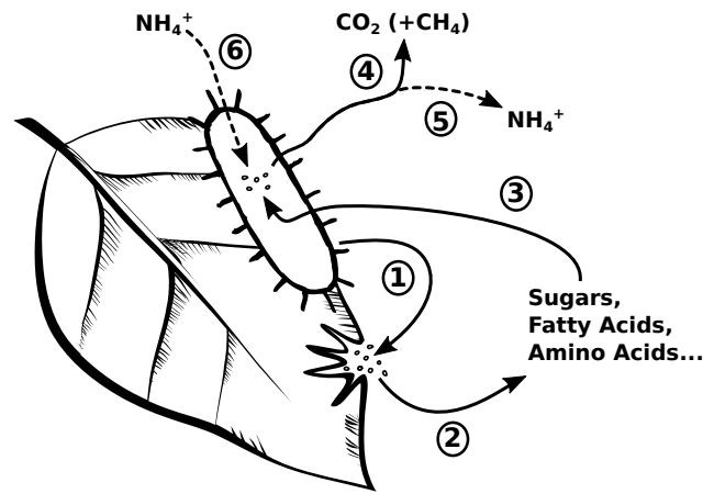
Figure 1. A conceptual view on c15 carbon (C) cycling and nitrogen (N) cycling during litter decomposition. Microbial decomposers release exoenzymes (1), which depolymerize plant biopolymers to soluble monomers (2). The relative distribution of formed monomers depends on plant tissue composition and specific enzyme activities. Microbial decomposers assimilate the monomers (3) and either use the contained organic matter for growth or to obtain energy c16 through mineralization (4). Microbial growth leads to an accumulation of microbial biomass within litter. N mineralization leads to a loss of ammonium to the environment (5), but this process is only active if amino acid-N supply (due to protein depolymerization) exceeds microbial N demand. Ammonium from the environment can additionally serve to fulfill microbial N demand (6).
