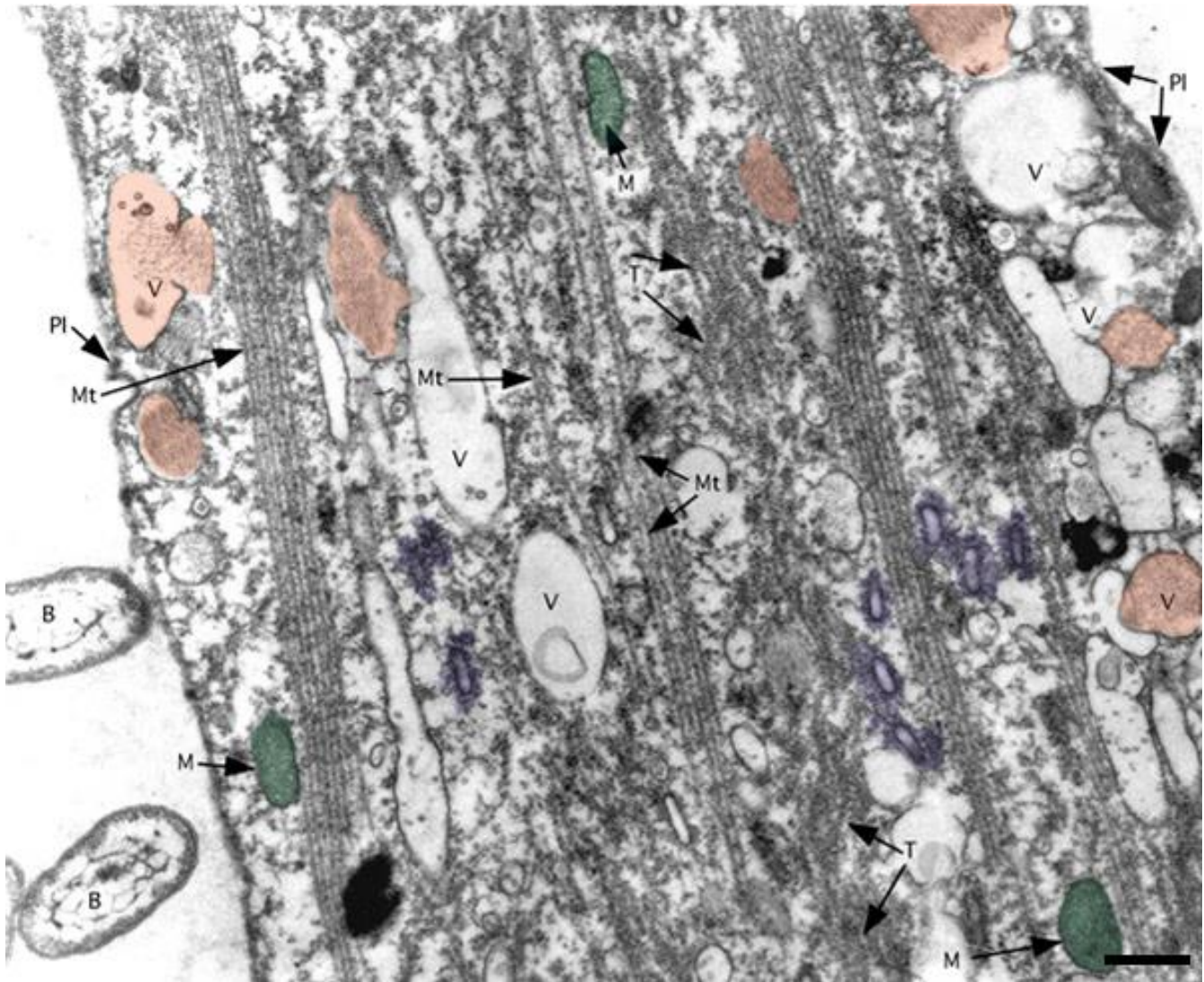
5 Figure 8. TEM image of ectoplasm of Assilina ammonoides (Gronovius) (modified from Hottinger, 2006, fig. 67 based on Creative Commons Attribution 2.5 License) Areas marked in red indicates vesicles we interpret as fibrillar vesicles. Areas marked in violet indicates what we interpret as Fuzzy coated vesicles also called Motility Organising Vesicles (MOVs). Green areas correspond to mitochondria. B: bacteria; M: mitochondria; Mt: microtubule; PI: plasmalemma; T: tubulin paracrystals; V: vacuoles with or without fibrillar content. Scale = 500 nm.
