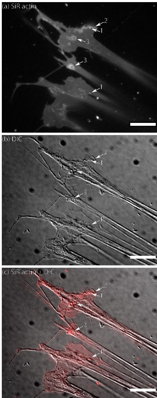
Figure 1: Flattened lamellipodia of living Ammonia sp. attached to glass: (a) fluorescence of SiR-actin-labelled structures, (b) DIC image of the same area, (c) merged image of fluorescence and DIC channels (since the reticulopodia were moving, the DIC image is slightly shifted in relation to fluorescent one). Numbers indicates: 1 – actin labelled granules (ALGs); 2 – linear SiR-actin-labelled structures; 3 – SiR-actin-labelled rings. Note weak but not uniform SiR-actin-labelling following all membranous surfaces of pseudopodial structures. The linear structure (2) was subsequently transformed into ring structure (see Movie S1 in Supplement). Structures corresponding to ALGs, SiR-actin-labelled ring and linear structures can be seen in DIC image. Conventional fluorescence images were obtained with Zeiss Axio Observer Z.1 . Scale bar 20 \mu m.
