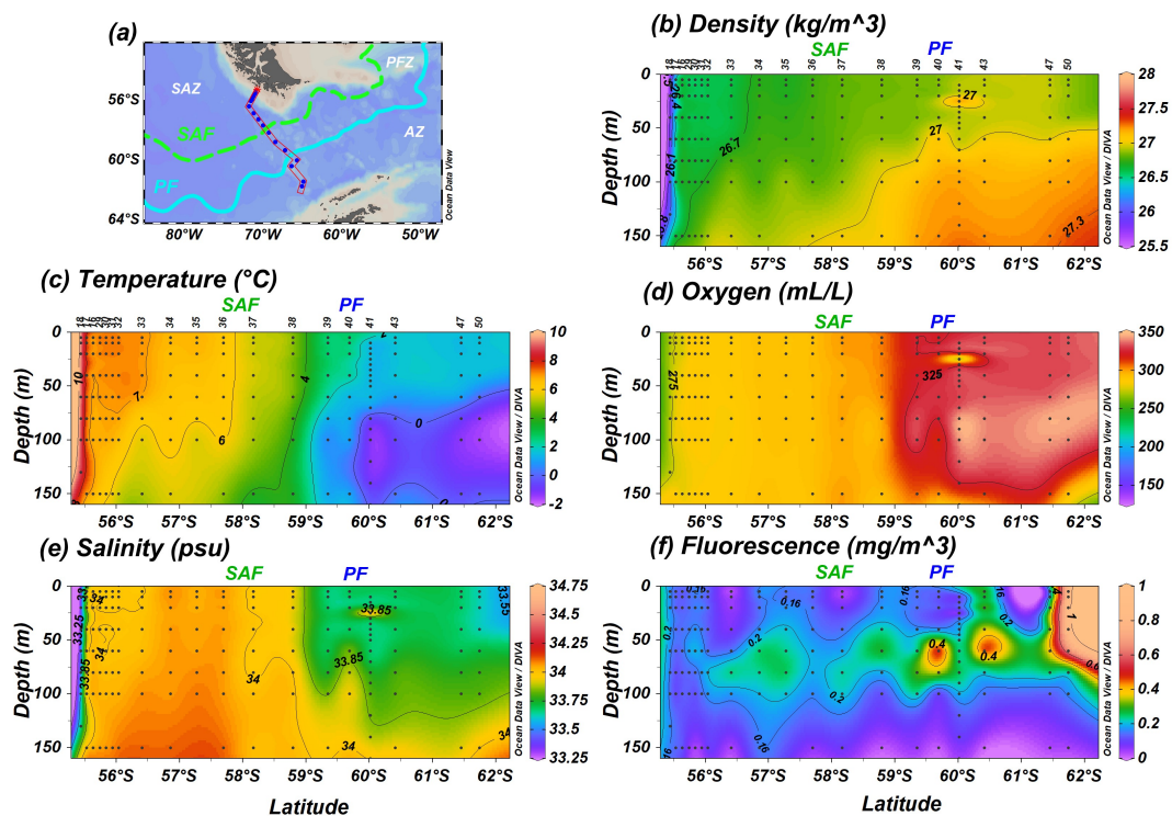
5 Fig. 2. (a) Location of the PS97 CTD stations studied, (b) water density ( \text{kg/m}^3 ), (c) sea surface temperature ( ^{\circ}\text{C} ), (d) dissolved oxygen ( \text{mL/L} ) (e) sea surface salinity (psu) and (f) fluorescence ( \text{mg/m}^3 ) profiles from 55.4°S to 61.7°S up to a depth of 150 m. Black dots indicate sampling points. The different oceanographic fronts (according to Orsi et al., 1995) are indicated as SAF—green dashed line, PF—blue line.
