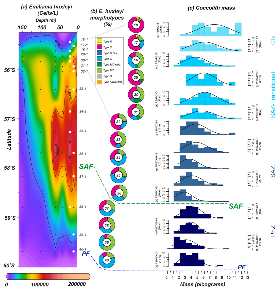
5 Fig. 11. (a) Location of the PS97 CTD stations between 55.4 and 60°S showing the number of cells/L of Emiliana huxleyi from 0 to 150 m. (b) Relative abundance of E. huxleyi morphotypes (including the different degree of calcification observed in SEM) in a latitudinal transect (10–20 m, indicated with white dots in (a)), and (c) coccolith mass histograms at those specific locations. Bin size in (c) is 1 picogram and normal distribution fitting line is shown. Station's number, different zones: Chi (Chilean coastal zone), SAZ-Transitional (from Chi to open ocean), SAZ (subantarctic zone), PFZ (polar front zone), and the main oceanographic fronts: Subantarctic (SAF) and Polar Fronts (PF) according to Orsi et al. (1995) are indicated.
