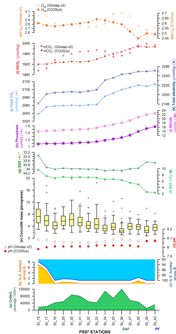
5 Fig. 12. Latitudinal transect showing on the left hand side: (a) the uppermost 150 m average of cells/L, relative abundance of E. huxleyi morphotypes belonging to (b) group A and (c) to group B, (d) pH calculated with different approaches (Pierrot et al., 2006; Key et al., 2015), (e) coccolith mass boxplot (outliers have been indicated with “+”), (f) sea surface temperature (SST, °C) and (g) salinity (note the inverted scale) measured in situ (Lamy, 2016). Interpolated (h) phosphate (μmol/L) and (i) nitrate contents (μmol/kg) (Garcia et al., 2014), (j) total alkalinity (μmol/kg) and (k) total CO 2 (μmol/kg) (Goyet et al., 2000), (l) bicarbonate ion (HCO 3 - , μmol/kg) and (m) calcite saturation state (Ω ca ) calculated with different approaches (Pierrot et al., 2006; Key et al., 2015). The subantarctic (SAF) and Polar Fronts (PF) according to Orsi et al. (1995) are indicated.
