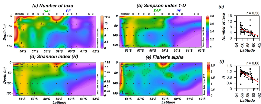
Fig. 9. PS97 latitudinal transects showing coccolithophore diversity: (a) number of taxa, (b) Simpson index 1-D, (c) number of taxa vs latitude, (d) Shannon index ( H ), (e) Fisher's alpha and (f) H vs latitude. The Subantarctic Front (SAF) and the Polar Front (PF) according to Orsi et al. (1995) are indicated.
