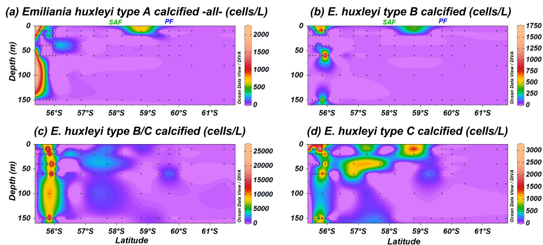
5 Fig. 10. Location of the PS97 CTD stations studied showing the number of coccospheres/L of Emiliana huxleyi calcified and overcalcified (a) type A group, (b) type B, (c) type B/C and (d) type C. The Subantarctic Front (SAF) and the Polar Front (PF) according to Orsi et al. (1995) are indicated.
