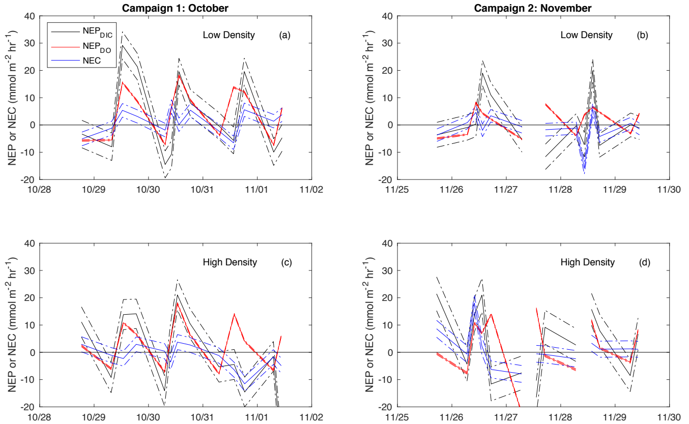
Figure 5. Time-series plot of NEC (blue), \text{NEP}_{\text{DIC}} (black) and \text{NEP}_{\text{DO}} (red), including the upper and lower uncertainty bounds related to error due to advection (dashed lines).
