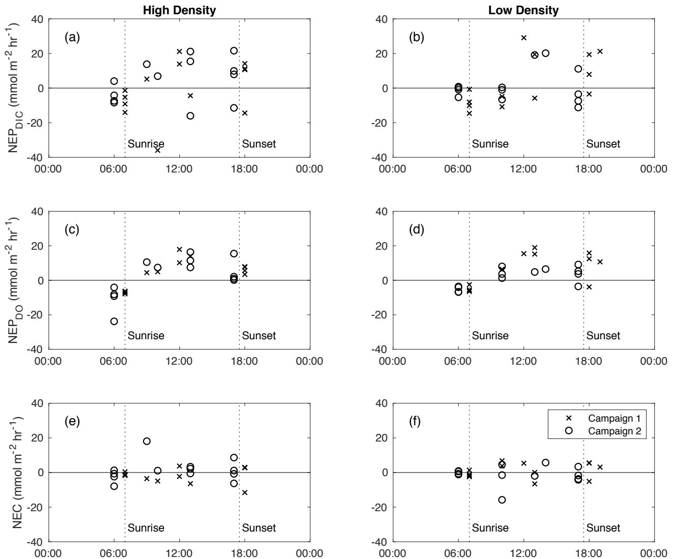
Figure 4. Diel trends in NEP DIC (a-b) and NEP DO (c-d) NEC (e-f), for the high-density site (left panels) and low-density site (right panels), for sampling campaign 1(X) and 2 (O). The x-axis represents the midpoint time for each NEP or NEC calculation period.
