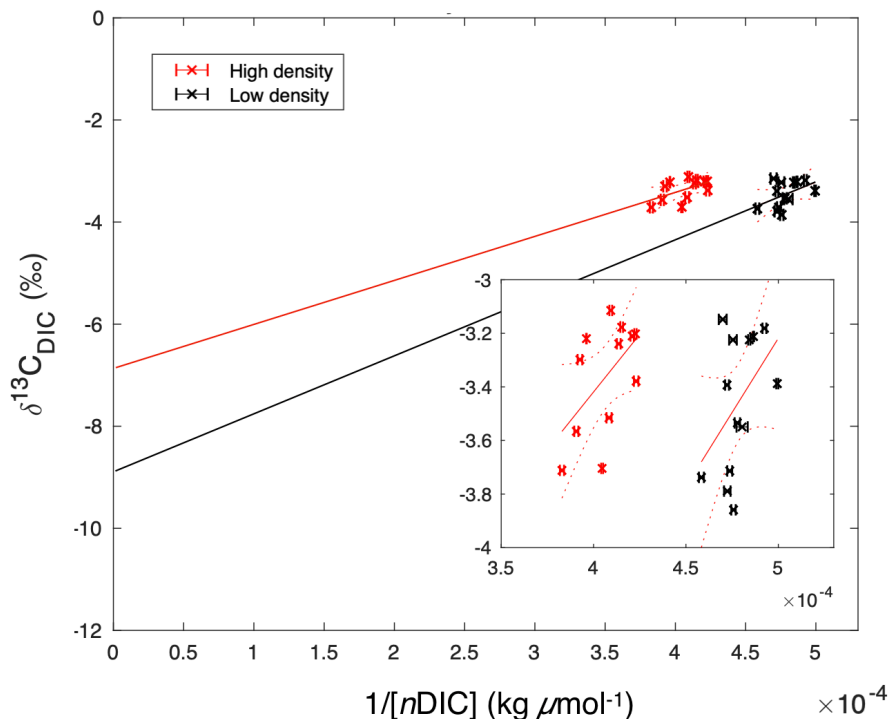
Figure 10. ‘Keeling plot’ of 1/[nDIC] versus \delta^{13}C_{DIC} , suggesting potential end-member isotopic values. These y-intercept \delta^{13}C_{DIC} values were -6.9 \pm 3.7 and -8.8 \pm 6.8 ‰ (95% confidence interval) for the high- and low-density sites respectively. The inset figure is zoomed to the extent of collected data, while the large figure is scaled to demonstrate the extrapolation required in order to extend the data to the y-intercept.
