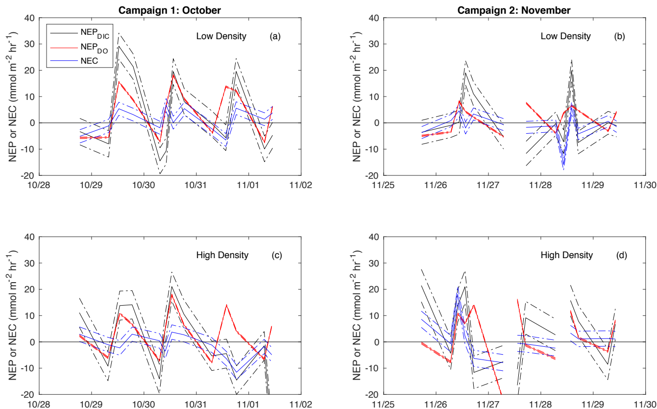
Figure 5. Time-series plot of NEC (blue), \text{NEP}_{\text{DIC}} (black) and \text{NEP}_{\text{DO}} (red), including the upper and lower uncertainty bounds related to error due to advection (dashed lines).
