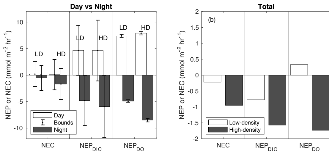
Figure 6. NEC, NEP_{DIC} , and NEP_{DO} integrated over day and night-time periods (a), and over the entire study period (b). NEP values are shown for k_{600} of Ho et al., 2006. The error bars in figure (a) represent upper and lower bounds for metabolic rates determined in section 2.8.
