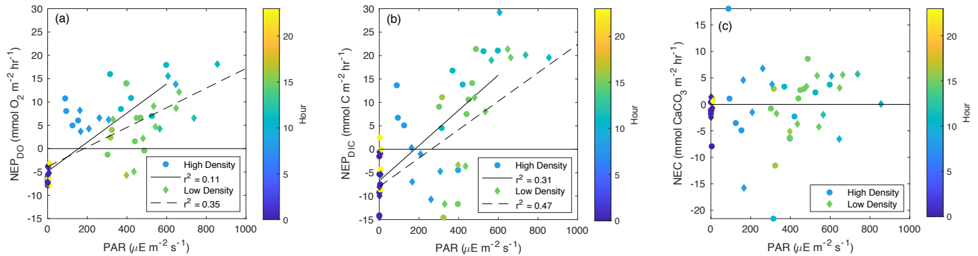
Figure 7. Scatter plots of (a) NEP_{DO} vs PAR, NEP_{DIC} , and NEC vs PAR (b-c). Points are colored by the average hour for the respective time period over which NEP or NEC was calculated. The arrows in (a) are intended to highlight the hysteresis pattern between PAR and NEP_{DO} .
