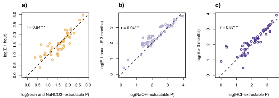
5 Figure 2. Correlation between chemically extracted pools and isotopically exchangeable P. Resin and NaHCO 3 -extractable P correlated with P exchangeable in 1 hour (E 1 hour) (a), NaOH-extractable P with P exchangeable between 1 hour and 3 months (b), and HCl-extractable P with P only exchangeable in over three months (c). Units of both axes are log(mg P kg -1 ). Dotted line shows the 1:1 line. Pearson's product-moment correlation ( r value on plot) was highly significant ( p < 0.001 ) for all three correlations.
