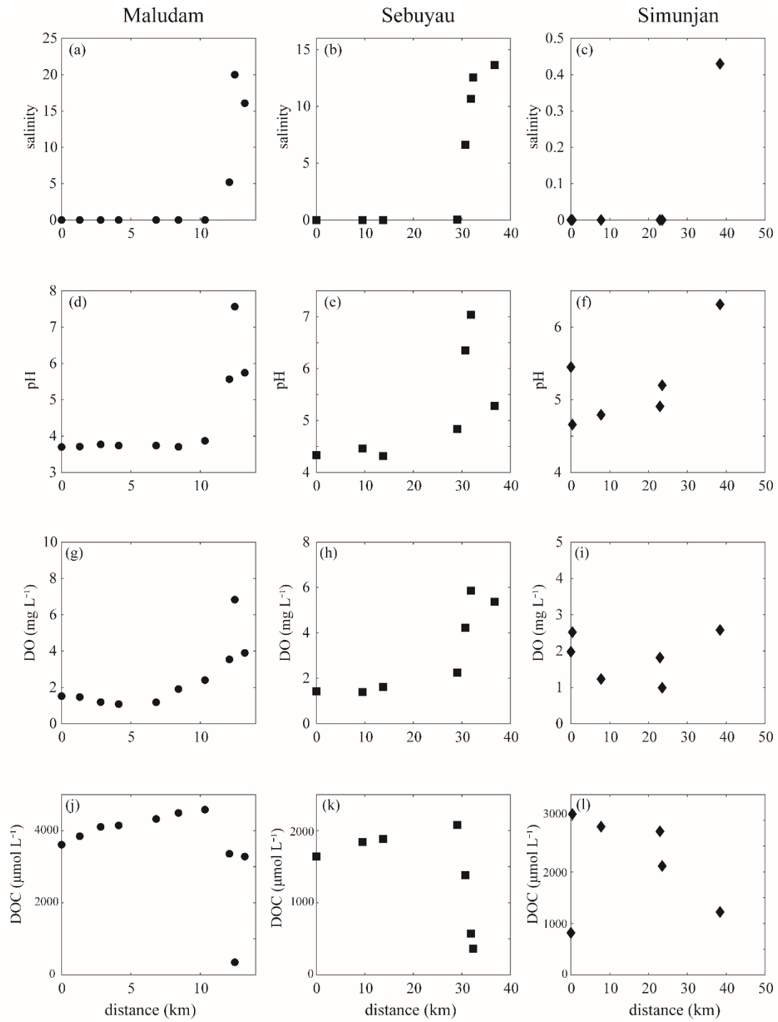
Supplement: The correlation of the distance with salinity (a-c), pH (d-f), dissolved oxygen (DO) (g-i), and dissolved organic carbon (DOC) (j-l) in blackwater rivers including Maludam, Sebuyau, and Simunjan. We adopted the station at the upper stream as distance=0, and the downstream direction as positive.
