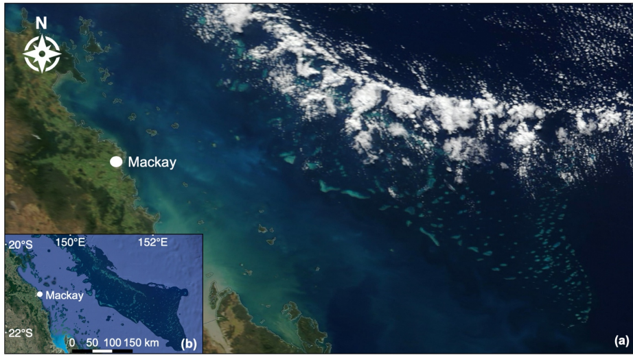
Figure 7. (a) Low-level convective clouds aligned over the Swains Reefs in the Mackay-Capricorn Management Area of the southern GBR. True colour image captured by MODIS Terra on 31 st May 2018 (NASA Earth Observing System Data and Information System). (b) Map of the southern GBR shown to be covered by clouds in the true colour image (map data ©2019 Google).
