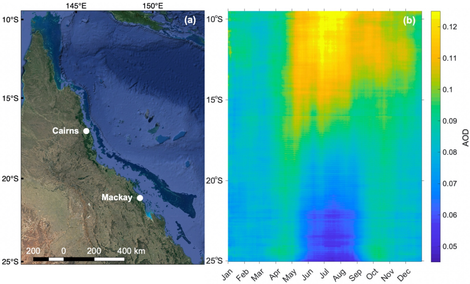
Figure 6. (a) Map of the GBR, Australia (map data ©2019 Google), showing the region defined in (b) longitude-averaged Hazy-moller plot of daily mean (2001 - 2017) total AOD (869 nm) over the GBR.
