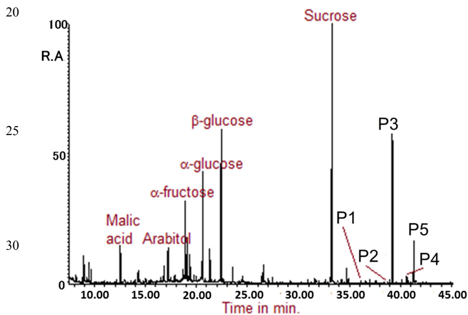
35 Figure 2: GC-MS total ion chromatogram obtained for the TMS derivatives. P1–P5 refer to peaks, which correspond to the secondary fatty alcohols identified in this study.
