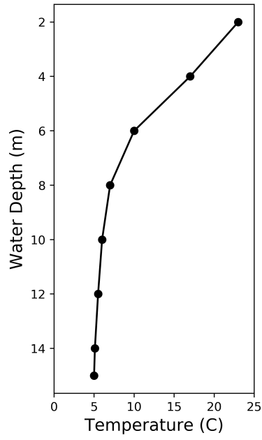
Fig. 1. Figure S3. Water temperature profile taken during June 16, 2018 sampling event on Upper Mystic Lake.
