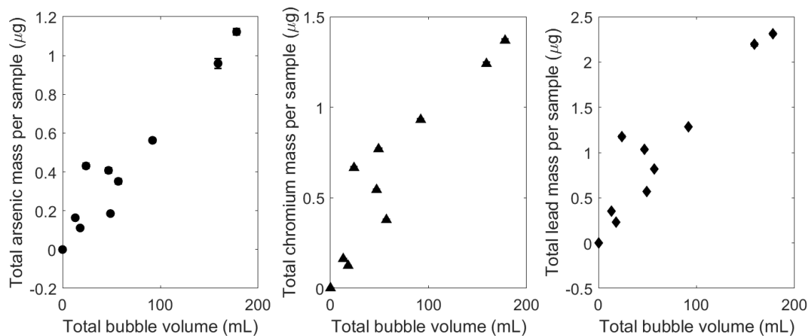
Figure 4: Chemical amounts observed in bubble traps associated with bubble-mediated transport of sediment particles. (a) Arsenic mass, (b) chromium mass, (c) lead mass (in \mu\text{g} ) transported versus the bubble volume of each sample (in mL, as measured at the lake surface a-c). Standard deviation is added to each measurement but the scale similar to point size for most measurements.
