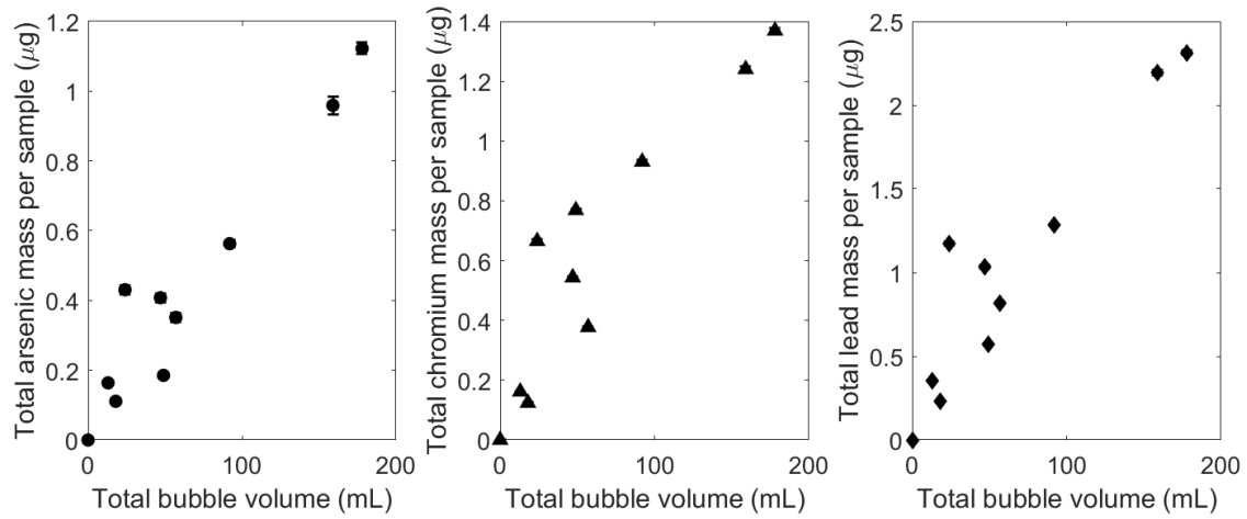
Figure 4: Chemical amounts observed in bubble traps associated with bubble-mediated transport of sediment particles. (a) Arsenic mass, (b) chromium mass, (c) lead mass (in µg) transported versus the bubble volume of each sample (in mL, as measured at the lake surface a-c). Standard deviation is added to each measurement but the scale similar to point size for
