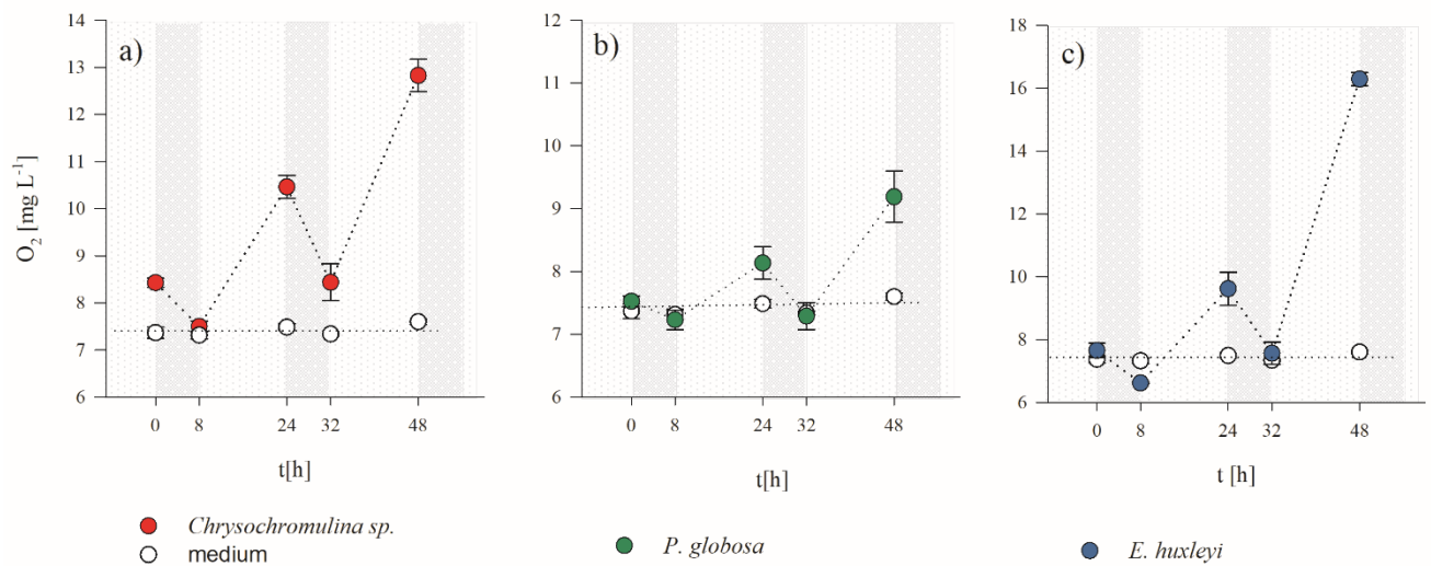
S2: Dissolved oxygen concentration in dark and light periods of three algae species Chrysochromulina sp. , P. globosa and E. huxleyi . Mean values of four replicated culture experiments are shown and error bars mark the SD. White and grey shading mark the light and dark periods.
