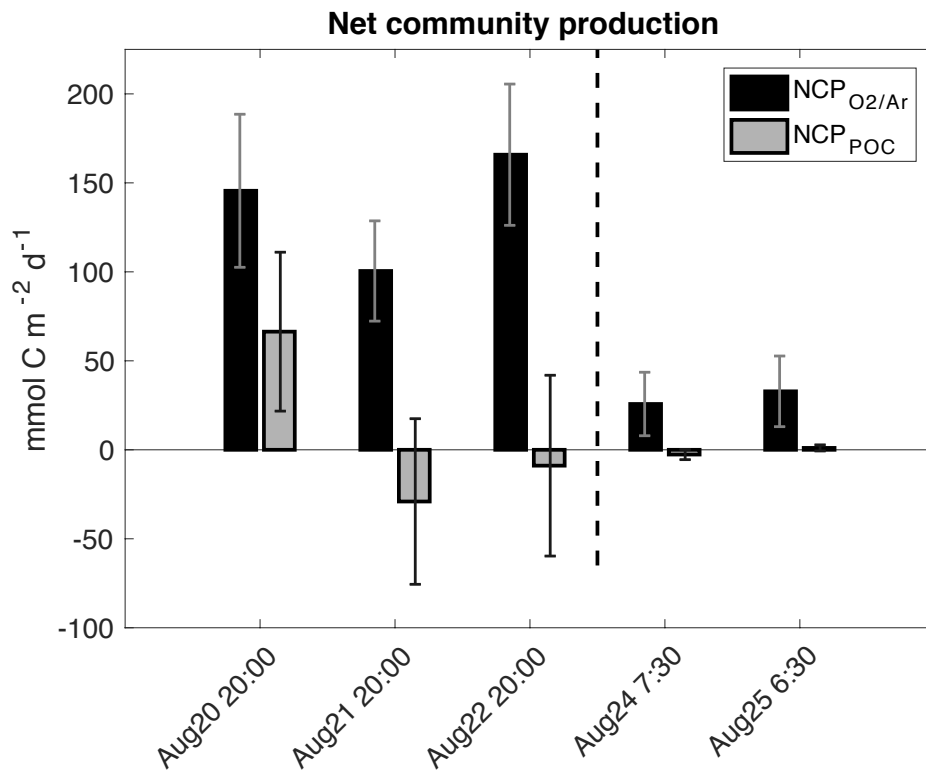
Fig. 1. Daily net community production (NCP)
