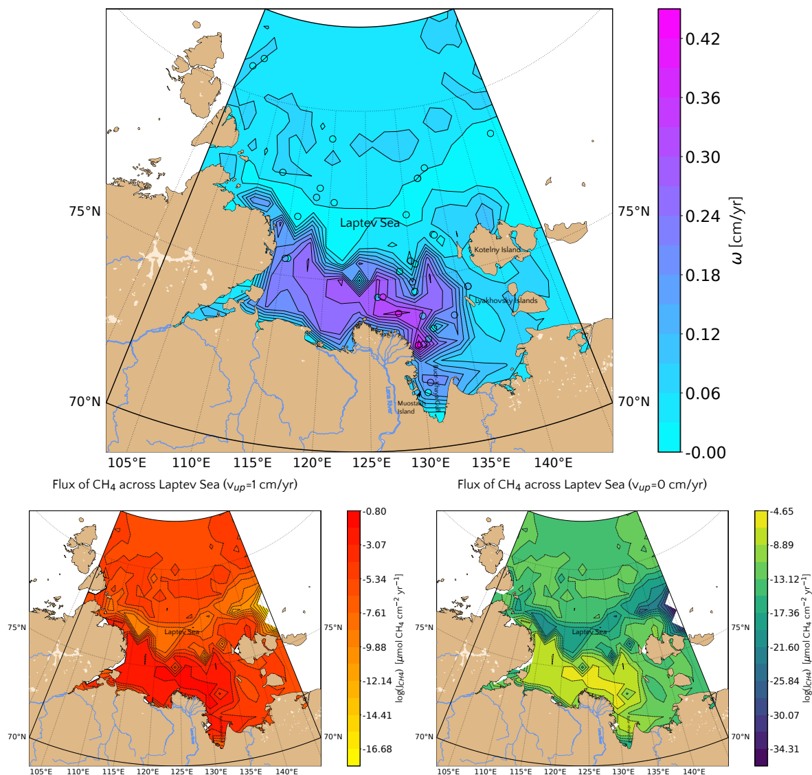
Figure 9. a. values of the sedimentation rate extrapolated for the whole Laptev Sea via a simple kriging method. The reference values (circles) are the ones reported in Table S8. Bottom (Log) Values of the potential methane emissions at the SWI considering the relationship presented in Fig. 3.c for passive ( b ) and active ( c ) cases.
