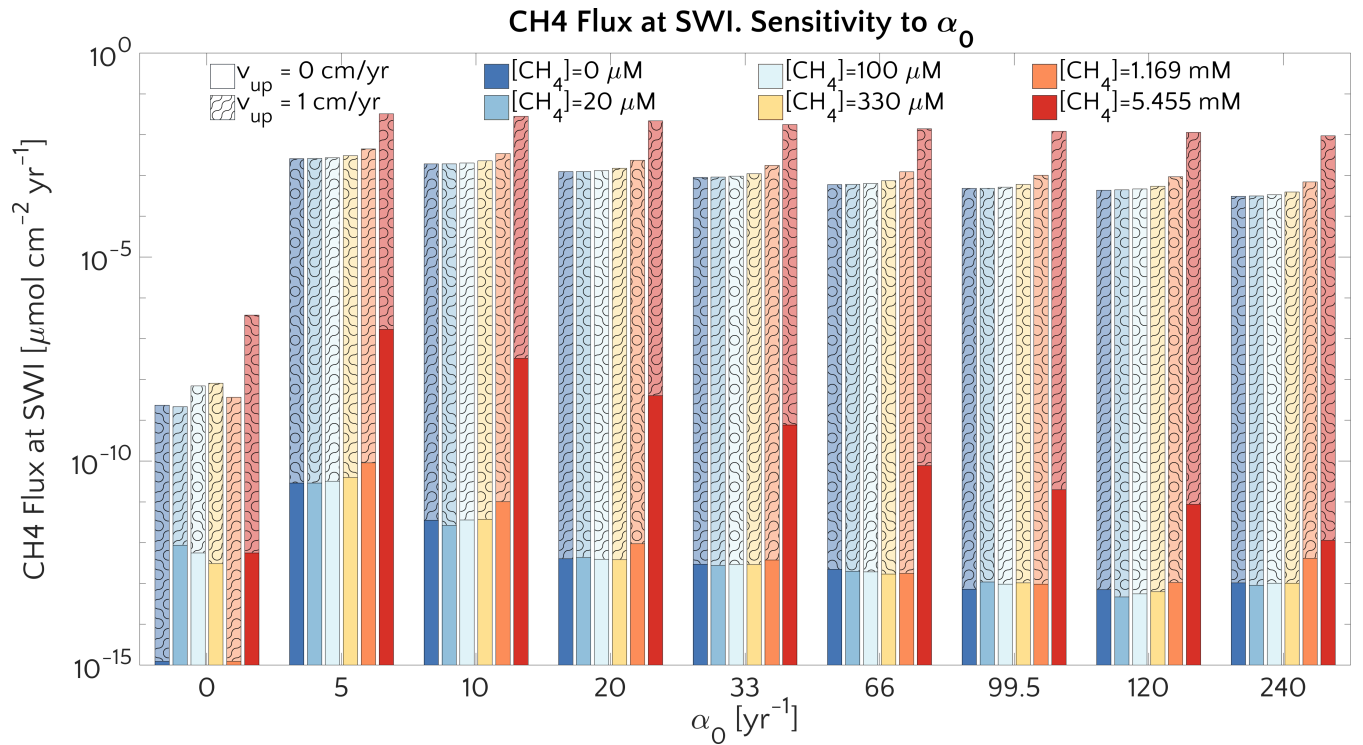
Figure 7. Barplot of the methane flux at the SWI versus \alpha_0 for passive case (plain style) and active case (pattern style) and the [\text{CH}_4] reported in the text.
