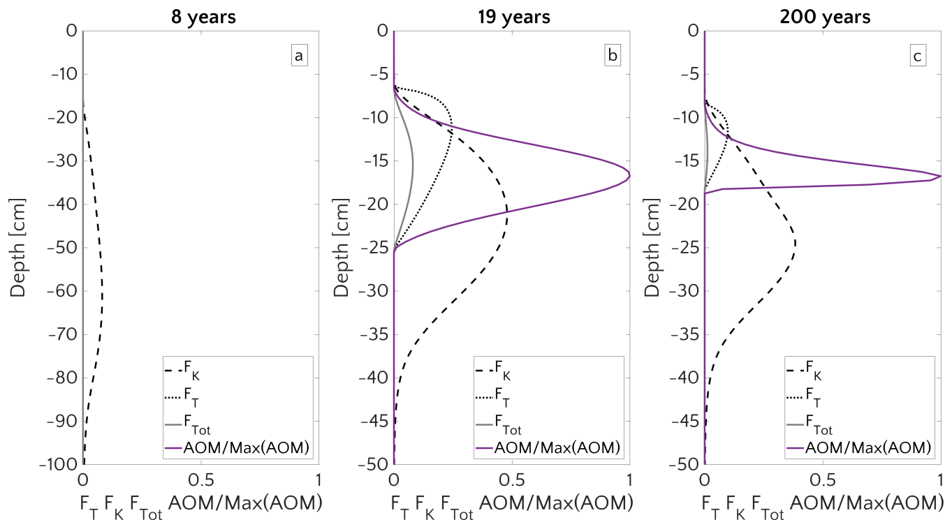
Figure 12. Vertical profile of F_T , F_K , F_{Tot} = F_K \cdot F_T and the AOM (scaled to the maximum) for three instant in times. 8 years (a), 19 years (b) and 200 years ((c) of simulation, for the case [\text{CH}_4]_- = 1.169 \text{ mM} and v_{up} = 5 \text{ cm yr}^{-1} .
