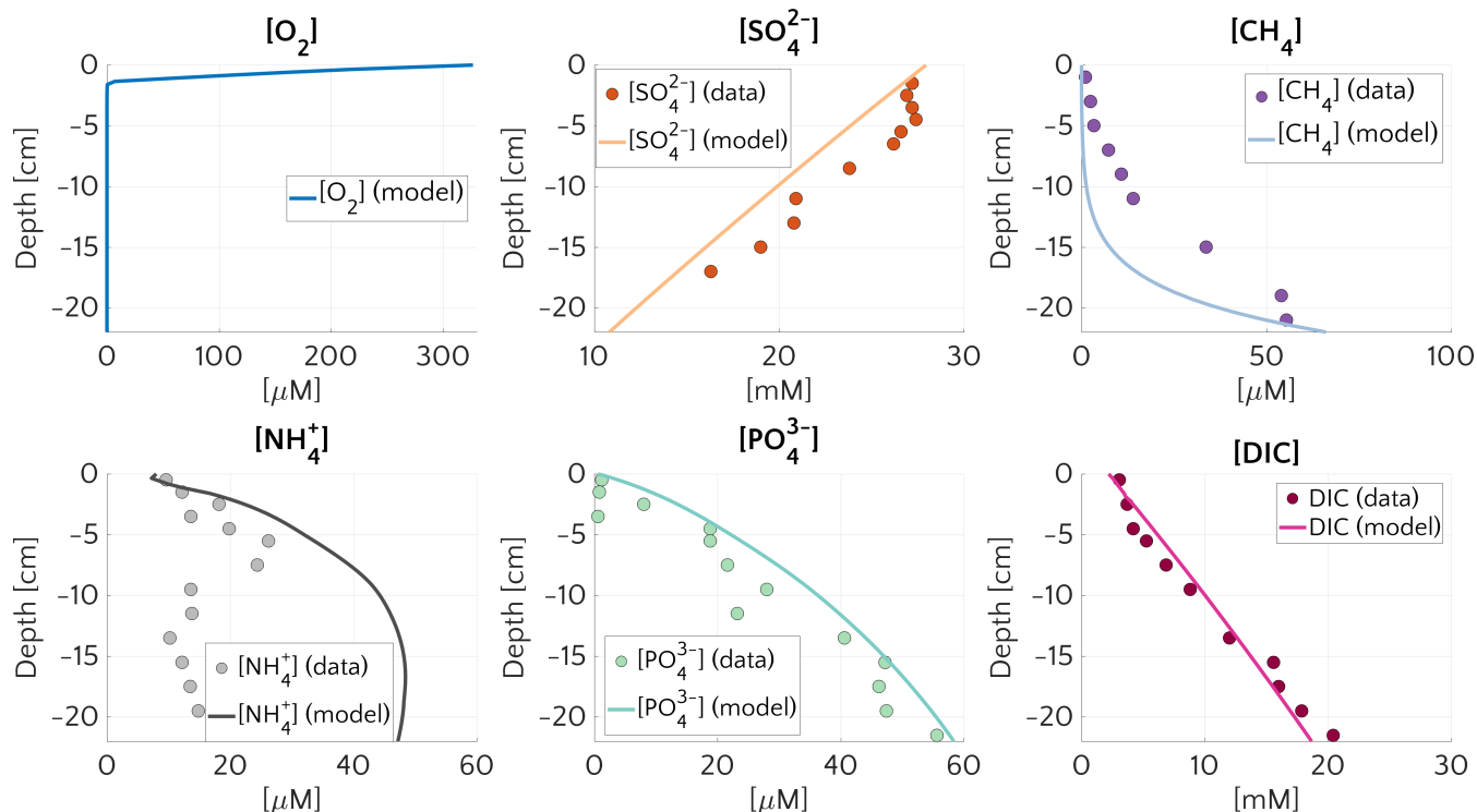
Figure 1. Pore water concentration profiles for O_2 , SO_4^{2-} , CH_4 , NH_4^+ , PO_4^{3-} and DIC at site 14-3 on the Laptev Sea (76.171°N, 129.333°E, 56 m water depth). Dots represents the measurements and continuous lines the simulated results. The boundary conditions and model parameters employed in the model are reported in table S4, the measured organic carbon content in table S5. For O_2 no measured profile is available.
