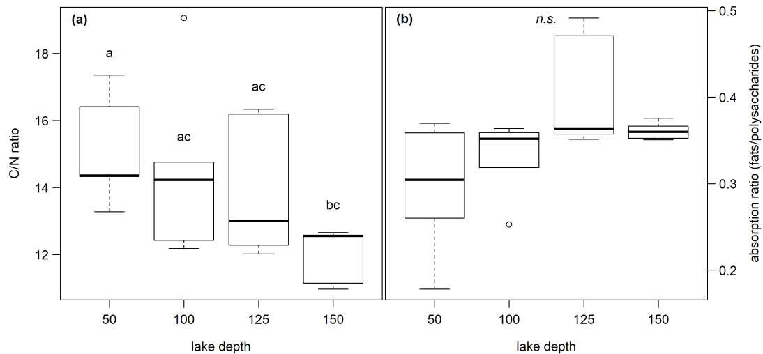
Fig. 1. C/N and FTIR peak ratio vs. lake depth category (see comment on ll. 545-556)
