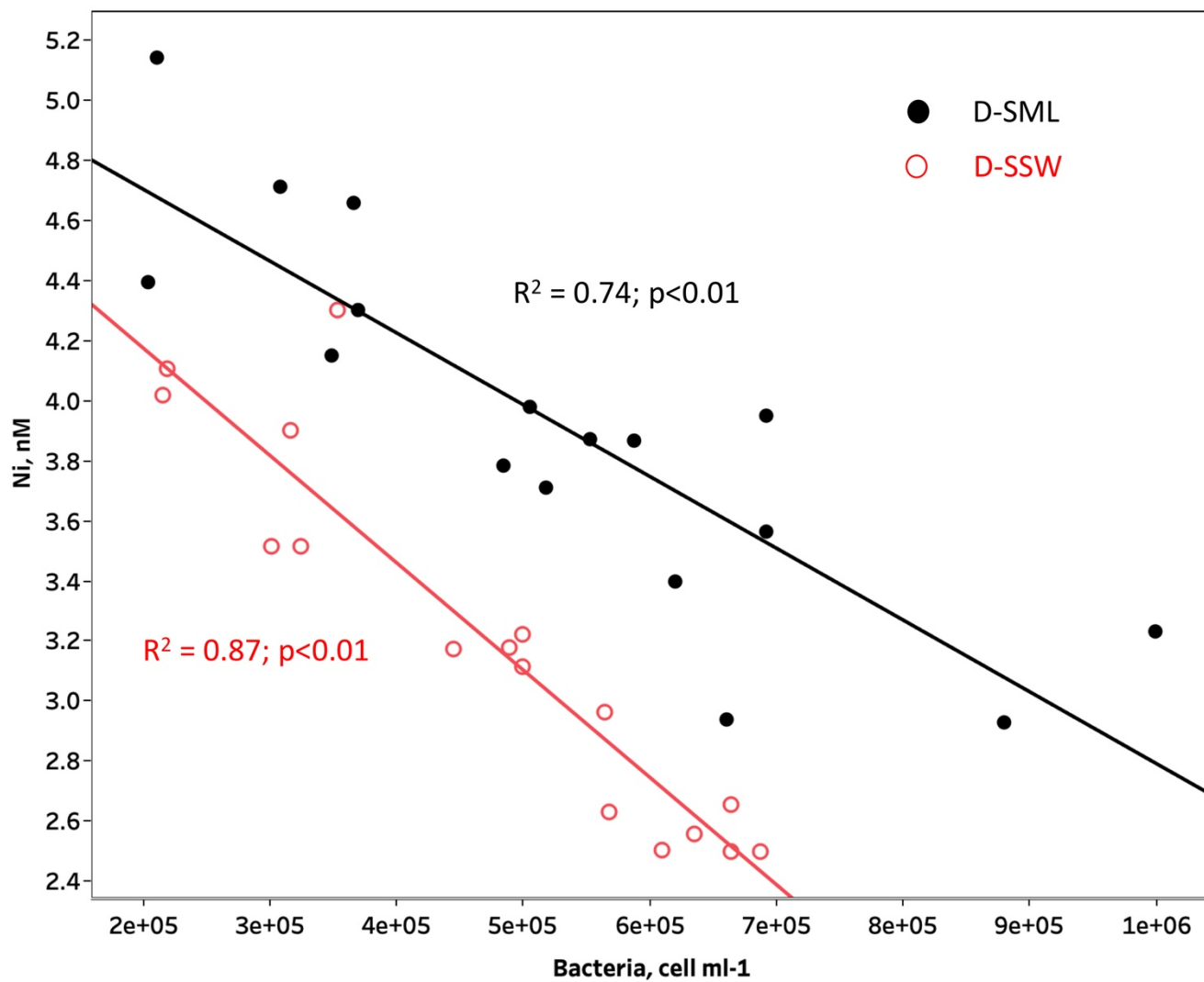
Figure 2. Concentration of dissolved Ni plotted against bacterial abundance in both the surface microlayer (SML, black dots) and the subsurface water (SSW, red open dots). The lines represent least square linear regressions.
