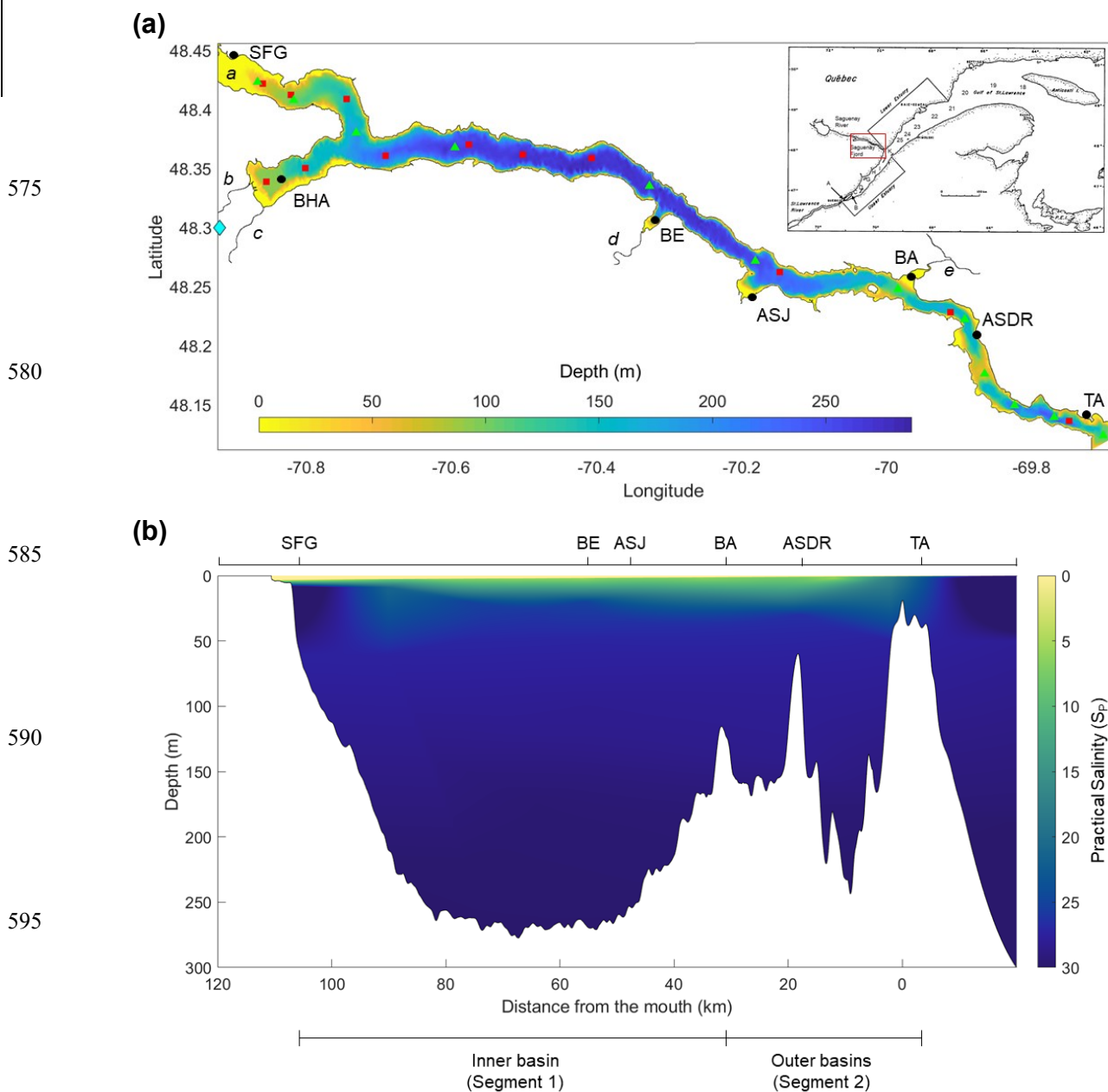
Figure 1. a) Bathymetry and geographic location of the Saguenay Fjord. Red squares represent the hydrographic stations sampled during R/V Coriolis II cruises in September 2014, May 2016, June 2017 and May 2018. Green triangles represent the hydrographic stations sampled during a SECO.net cruise onboard the R/V Coriolis II in November 2017. The approximate locations of the following are shown: Tadoussac (TA), L'Anse de Roche (ASDR), Baie Sainte-Marguerite (BA), Anse-Saint-Jean (ASJ), Baie-Eternité (BE), St. Fulgence (SFG), Baie des Ha! Ha! (BHA). The main tributaries to the fjord are also shown, including the Saguenay River (a), Rivière-à-Mars (b), Rivière des Ha! Ha! (c), Éternité River (d) and Sainte-Marguerite River (e). The blue diamond identifies the location of the La Baie weather station. Letters (A to K) and numbers (18 to 25) in the inset indicate the location of sampling stations in the St. Lawrence Estuary where data were acquired to define the SLRW, LSLE and CIL end-members. b) Longitudinal section along the Saguenay Fjord, showing the strong halocline.
