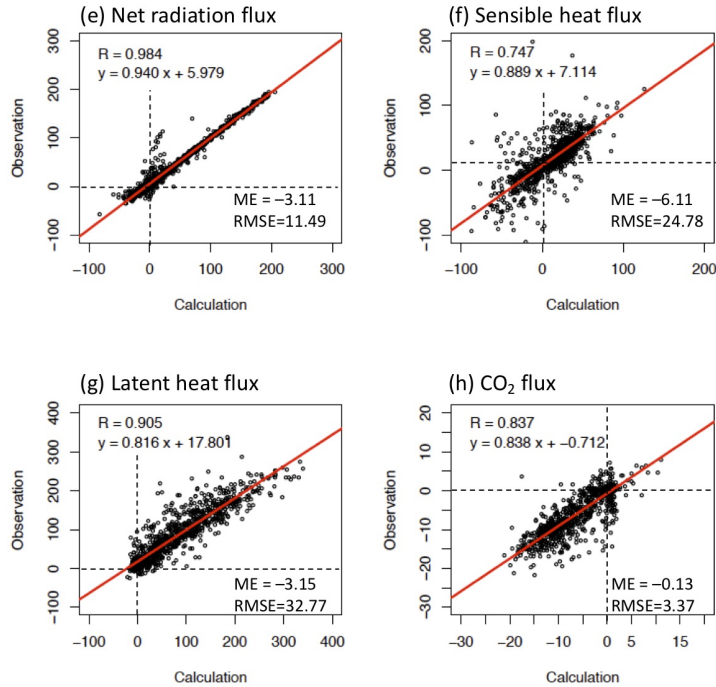
Figure 3. Scatter diagrams of calculated and observed (a, e) daily mean net radiation ( R_{net} ), (b, f) sensible ( H ) and (c, g) latent ( \lambda E ) heat, and (d, h) CO 2 fluxes ( F_{CO_2} ) at (a-d) Fendt and (e-h) Graswang for the study period.
