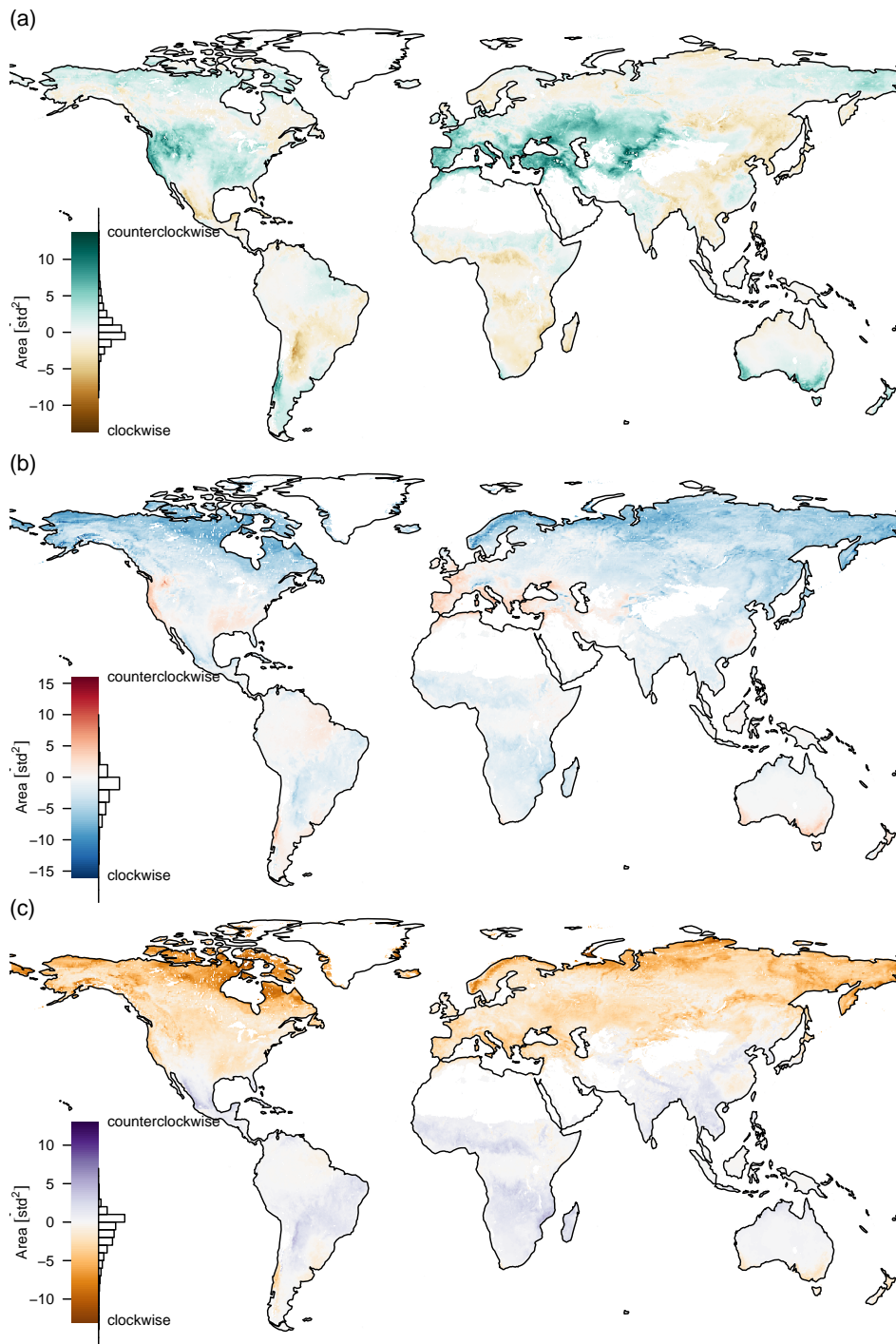
Figure 7. The area inside the mean seasonal cycles of (a) PC_1-PC_2 , (b) PC_1-PC_3 , and (c) PC_2-PC_3 . The area is positive if direction is counterclockwise and negative if the direction is clockwise. Most of the trajectories need a strong seasonal cycle to show a pronounced hysteresis effect. If the mean seasonal cycle intersects, the areas cancel each other out, e.g. the green trajectory of 4b.
