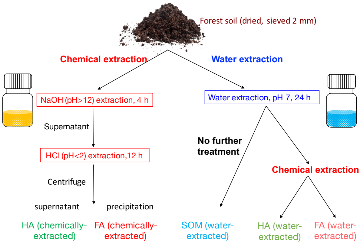
Figure 1. Schematic diagram of soil organic matter (SOM) extraction process. Forest soil samples (Schönbuch forest, Baden-Wuerttemberg, Germany) were dried under 30 °C and ground grinded to pass 2 mm sieve. To chemically extraction ion FA and HA, 100 g soil was incubated with 400 mL 0.1 M NaOH (pH 12) for 4 h, after centrifugation, the supernatant was acidified by HCl to pH < 2, HA was then precipitated out to be separated from FA. For water extraction, 100 g soil was incubated with 400 mL ultra-pure doubly-deionized water (<18.2 MΩ.cm; Milli-Q, Millipore) at pH 7. pH was monitored during the extraction and it remained stable (range between 7.02-7.33). The slurry was centrifuged after 24 h; we define the supernatant as water extract. A 200 mL aliquot of the supernatant containing the water-extracted SOM was amended with 1 M NaOH until pH 12. After 4 h of incubation, the pH of the solution was adjusted to < 2 by 6 M HCl to precipitate HA and to separate FA. This extraction was conducted under both oxic and anoxic conditions.
