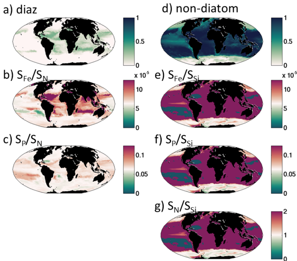
1060 Figure 13: Co-existence of functional types defined by imbalance of different nutrient supply rates. Left column depicts controls on diazotroph distribution: (a) fraction of total biomass made up of diazotrophs; (b) ratio of iron to DIN supply rates (see Fig 10); (c) ratio of phosphate to DIN supply rate. Colour scale is chosen such that purple indicates supply rate ratios in excess of the non-diazotroph Fe:N and P:N requirements. Right panel for co-existence of diatoms and non-diatoms: (d) fraction of biomass made up of non-diatoms; (e) ratio of iron to silicic acid supply rates; (f) ratio of phosphate to silicic acid supply 1065 rate, (g) ratio of DIN to silicic acid supply rates. Colour scale is chosen such that purple indicates supply rate ratios in excess of the diatom Fe:Si, P:Si, and N:Si requirements.
