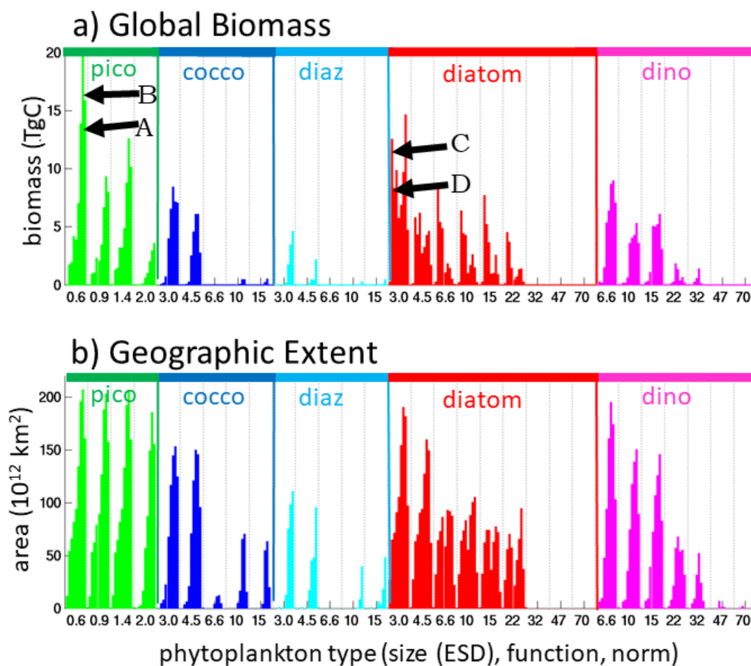
995 Figure 6: Model phytoplankton types biomass and range. (a) Global integrated biomass (TgC); (b) Areal extent of the type ( 10^{12} km 2 ). Types are arranged by functional group as indicated by the colour bar and labels at the top of the graph, by size classes (equivalent spherical diameter, ESD) as labelled below the graph, and thermal norms from cold adapted to warm adapted from left to right in between vertical dotted lines. The text (A,B,C,D) in panel (a) refers to representative types whose distributions are shown in Supplemental Fig 4.
