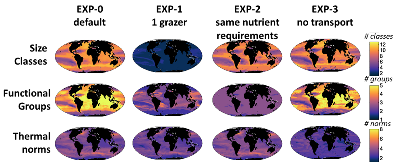
Figure 11: Sensitivity simulations, model annual mean richness for trait dimensions. EXP-1 has no size-dependent loss rates (i.e. only one grazer); EXP-2 has no nutrient requirement differences between functional groups; EXP-3 has no transport of the plankton (all nutrients and non-living organic pools are still transported). Top row: size class richness determined by number of co-existing size classes; Middle row: functional richness determined by number of co-existing biogeochemical functional groups; Bottom row: thermal richness determined by number of co-existing temperature norms. The left most column are the same output as shown in Fig 9b,c,d for the original (“default”) experiment.
