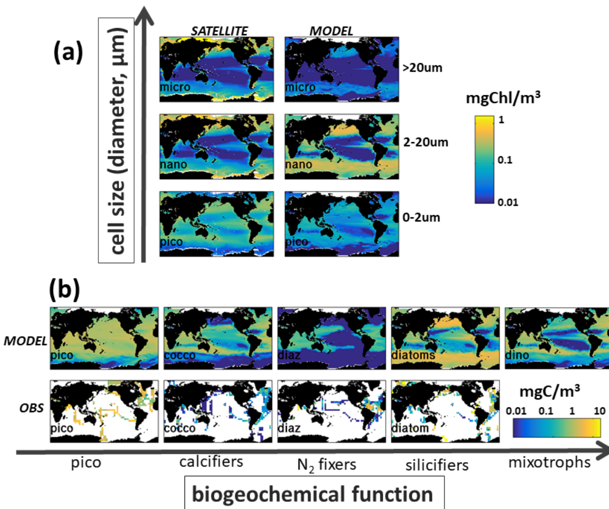
Figure 7. Comparison to Observations. (a) Sizes Classes: Chl-a concentration ( \text{mg Chl/m}^3 ) in pico ( <2\mu\text{m} ), nano ( 2\text{-}20\mu\text{m} ) and micro ( >20\mu\text{m} ) phytoplankton from (left) a satellite derived estimate (Ward, 2015) and (right) default model (0-50m); and (b) Functional groups (top) default model (0-50m) and (bottom) data compilation (MAREDAT, Buitenhuis et al 2013) in carbon biomass ( \text{mgC/m}^3 ). Note the difference in units for (a) and (b) which are chosen to match the appropriate observations. For the MAREDAT databases: pico-phytoplankton (Buitenhuis et al 2012); coccolithophores (O'Brien et al 2013); diazotrophs (Lou et al 2012); diatoms (LeBlanc et al 2012). There was no MAREDAT dataset for dinoflagellates.
