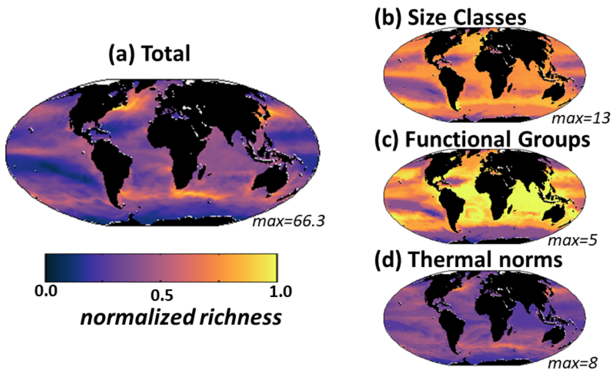
1010 Figure 8: Model diversity measured as annual mean normalized richness in the surface layer. Normalized is by the maximum value for that plot (value noted bottom right of each panel). (a) total richness determined by number of individual phytoplankton types that co-exist at any location; (b) size class richness determined by number of co-existing size classes; (c) functional richness determined by number of co-existing biogeochemical functional groups; (d) thermal richness determined by number of co-existing temperature norms. Total richness (a) is a (complex) multiplicative function of the three sub-richness 1015 categories (b-d).
