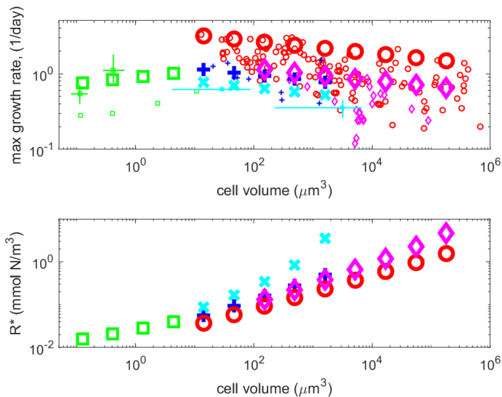
970 Figure 4: Model Parameters guide by laboratory studies. Phytoplankton maximum growth rate (top) and R^* (bottom) as a function of cell size. In (a) small symbols indicate laboratory studies normalized to 20° C, large symbols indicate the model size/functional groups. Colour of symbols denotes different functional groups: red circle=diatoms; purple diamond=mixotrophic dinoflagellates; dark blue plus=coccolithophores; light blue cross=diazotrophs; green square=pico- phytoplankton. In (b), R^* = \frac{k_R M}{\mu_{max} - M} , where M=0.5 1/d (see appendix). Data compilations of concurrent size and growth in (a) 975 are from Tang (1995); Maranon et al. (2013); Sarthou et al (2005); Buitenhuis et al (2008). Additional data are derived from separate measurement of size and growth: These are shown as light lines centered at the mean and arms covering range. These are for the pico-prokaryotes (green) Prochlorococcus and Synechococcus (Morel et al., 1993, Johnson et al. 2006, Christaki et al. 1999, Moore et al. 1998, Agawin and Agustí 1997) and the diazotrophs (light blue) Crocosphera and Trichodesmium 980 2008; Hutchins et al 2007; Kranz et al., 2010; Shi et al, 2012).
