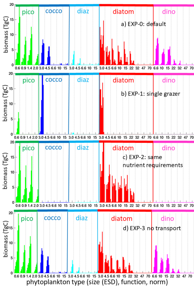
Figure 10: Sensitivity Experiments, phytoplankton global biomass. Global integrated biomass (TgC) for (a) default experiment (identical to Fig 3a); (b) EXP-1 (experiment with single generalist grazer); (c) EXP-2 (experiment where all phytoplankton have same nutrient requirements); (d) EXP-3 (experiment where phytoplankton are not transported). Types are arranged by functional group as indicated by the colour bar and labels at the top of the graph, by size classes (equivalent spherical diameter, ESD) as labelled below the graph, and thermal norms from cold adapted to warm adapted from left to right
