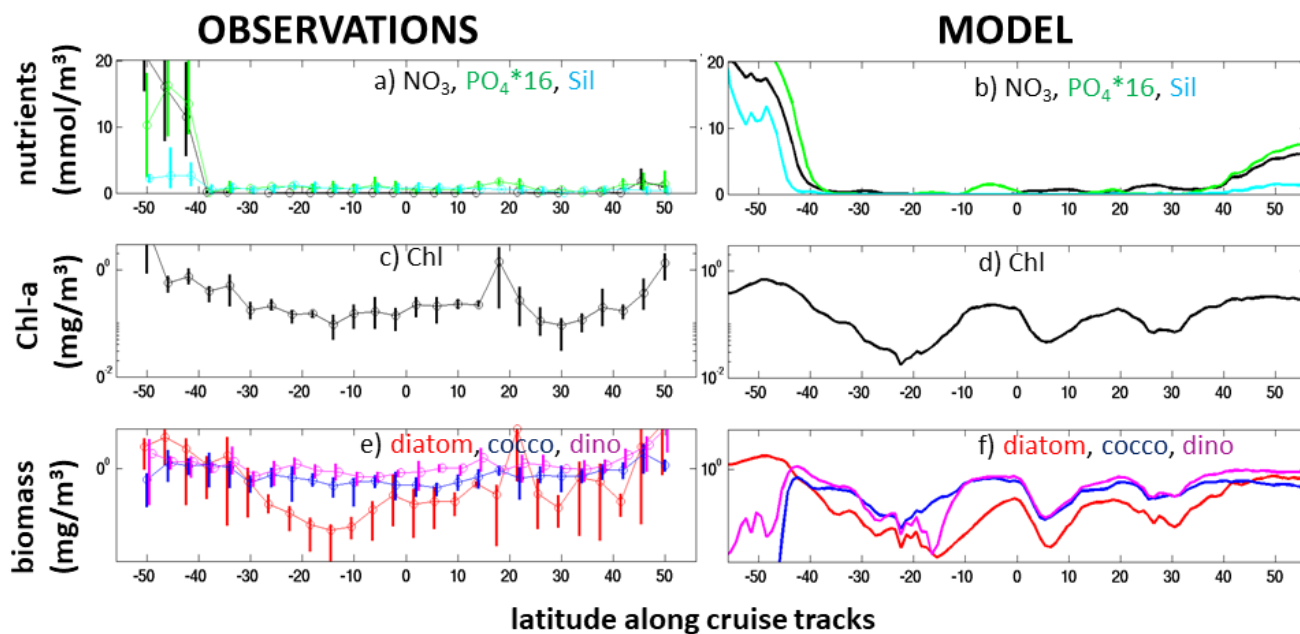
Figure 5: Observations and model output along the Atlantic Meridional Transect (AMT). (a), (b) nutrients (black=nitrate, \text{mmolN/m}^3 ; green=phosphate, 16\text{mmolP/m}^3 ; light blue=silicic acid, \text{mmolSi/m}^3 ); (c), (d) Chl-a ( \text{mg Chl/m}^3 ); (e), (f) phytoplankton biomass ( \text{mg C/m}^3 ; red=diatoms; blue=coccolithophores; purple=dinoflagellates). Observations (left panels) are mean (circles) for the 4 AMT cruises (2 in May, 2 in September, see methods) in 4^\circ bins, the vertical lines show the range within each bin. Model results are annual mean along the AMT cruise track.
