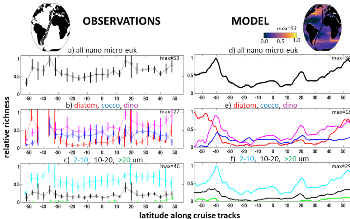
Fig 1: Nano- and micro-eukaryote normalized richness in the Atlantic. Left: richness (number of co-existing species) normalized to the maximum along the Atlantic Meridional Transects (AMT) 1,2,3,4 for microscopy counts (see methods). Right: normalized annual mean richness from model. (a),(d) all diatoms, coccolithophores and dinoflagellates together; (b),(e) each functional groups separately (red: diatoms, dark blue: coccolithophores, purple: dinoflagellates); (c),(f) 3 size classes (light blue: 2-10 \mu m, black: 10-20 \mu m, green: <20 \mu m). In left panels, circles are mean of four transects (2 in May, 2 in September) within 4° latitude bins, the vertical lines indicate the range within each bin. The maximum number used to normalise the plots are provided in each panel. Model pico-phytoplankton and diazotrophs are not included in the model analysis as they were not included in the observations. Maps show the cruise track of the AMTs, and for the model includes the annual mean normalized richness of the diatoms, coccolithophores and dinoflagellates together.
