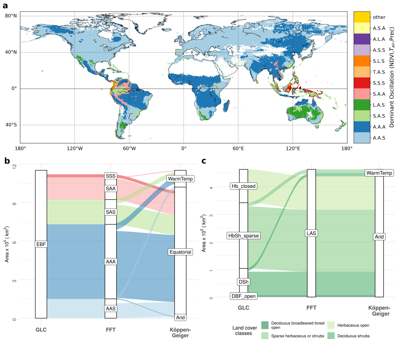
Figure 2. Classification of land surface by dominant scale of variability in NDVI and climate, and its relation to land cover and mean climate. a. Dominant scale of variability was determined for NDVI, T_{air} and Prec separately for each grid cell and summarized as unique combinations between variables (S – short-term, A – seasonal, L – longer-term, T – trend, listed in order NDVI, T_{air} , Prec). Only the 11 most common classes are shown. The semi-annual cycle is included in the seasonal band. b+c. Sankey diagrams (river plots) showing associations of pixels for (b) Evergreen broadleaf forest (EBF) and (c) regions of dominant long-term oscillations in NDVI (LAS class) to oscillation regime (FFT), land cover class (GLC2000) and Köppen–Geiger (KG) climate class. The width of the ribbons is proportional to the area that is commonly classified into the corresponding GLC2000, KG or oscillation classes. DBF: Deciduous broadleaf forest, Hb_closed: closed herbaceous land cover, DSh: deciduous shrublands, HbSh_sparse: sparse herbaceous and shrub vegetation, Equatorial: KG class A, Arid: KG class B, WarmTemp: KG class C.
