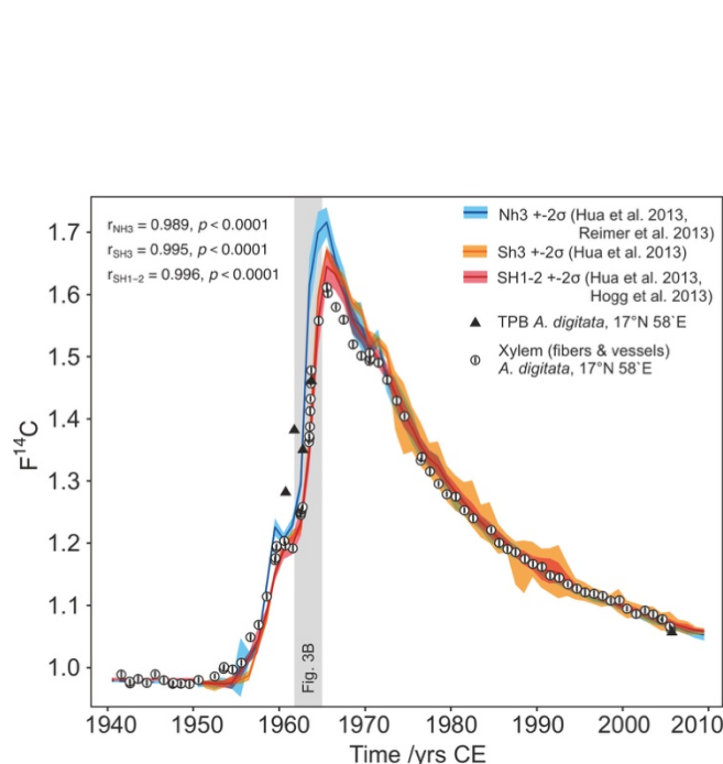
950 Figure 3: (A) Comparison of baobab F^{14}C values with F^{14}C curves for both hemispheres. Data prior to 1950 taken from IntCal13 and SHCal13 (Reimer et al., 2013, Hogg et al., 2013). 1950-2010 originates from Hua et al., 2013 (line: mean value, shade: \pm 2 standard deviations ( \sigma )). The southern hemispheric increase in atmospheric F^{14}C lags behind the northern hemisphere by about 1 year and its peak is considerably shallower. The overall conformity of the baobab measurements (white dots with 2\sigma error bar) with the course of the calibration curves proves the annual character of the growth zones. The values for baobab tree-ring cellulose (xylem fibers and vessels) lie between the values for both hemispheres for the steep increase in F^{14}C and then apparently follow the course of SH1-2, although temporary shifted due to different vegetation periods. Four out of five terminal parenchyma bands (TPB, black triangles, error bars are smaller than the symbol size) show either much higher F^{14}C values (1960-1962) or a lower value (2005) than the corresponding tree ring. (B) Baobab measurements in comparison to atmospheric (squares) and tree-ring data (circles) for NH3 (a-d), SH3 (e), and SH1-2 (f-i) between 1962 and 1964. These years show strongly increasing atmospheric F^{14}C values and were chosen to investigate the intra-annual baobab F^{14}C values. For this period, the baobab F^{14}C values lie between the higher NH3/SH3 and the lower SH1-2 values. A dip within the first half of the tree ring is followed by a slight (1962) or steep (1963) increase of the values. Note, the inter- and intra-species' variability from the same site (i.1 and i.2, Turney et al., 2018).
