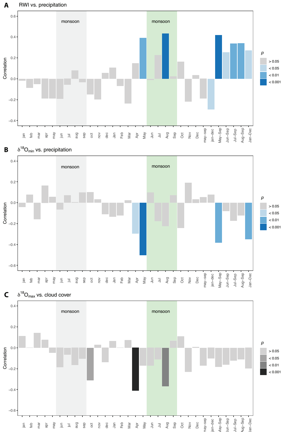
1030 Figure 7: Diagrams for the strongest correlations of baobab tree-ring parameters with monthly and seasonally resolved climate parameters. Months of the previous year are marked by lower case abbreviations, months of the current year by upper case abbreviations. The green box marks the average monsoon period. (A) Ring-width indices versus precipitation amount. (B) \delta^{18}\text{O}_{\text{min}} versus precipitation. (C) \delta^{18}\text{O}_{\text{max}} versus cloud cover. Apart from the actual monsoon season (Jun-Sep) also the pre-monsoon (Apr-May) has a significant influence on wood increment growth and \delta^{18}\text{O} isotope signature.
