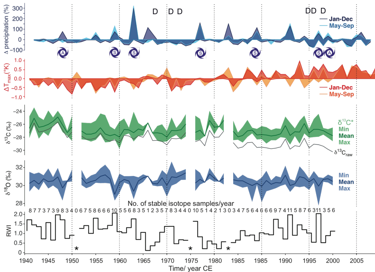
980 Figure 4: Analyzed baobab tree-ring parameters (ring width indices (RWI), \delta^{18}\text{O} , \delta^{13}\text{C}^* ) together with available precipitation and T_{\text{max}} data for the period 1941-2014. Precipitation is presented as percentage differences from the mean, T_{\text{max}} as differences in Kelvin. Darker colors reflect differences on an annual basis, lighter colors for the monsoon period Jun-September. The stable isotope values ( \delta^{13}\text{C}^* , \delta^{18}\text{O} ) are presented with minima, maxima and mean values for each year. Mean \delta^{13}\text{C} , uncorrected for effects of changing atmospheric \text{CO}_2 concentration and corresponding \delta^{13}\text{C}_{\text{CO}_2} is given as black line ( \delta^{13}\text{C}_{\text{raw}} ). Dry years with \leq 45 mm of rain during the monsoon period are marked with D. Years with spring (S) or autumn (A) storms with \geq 90 mm of rain are indicated by cyclone symbols. Missing rings caused gaps in the time series and are marked by asterisks. 985
