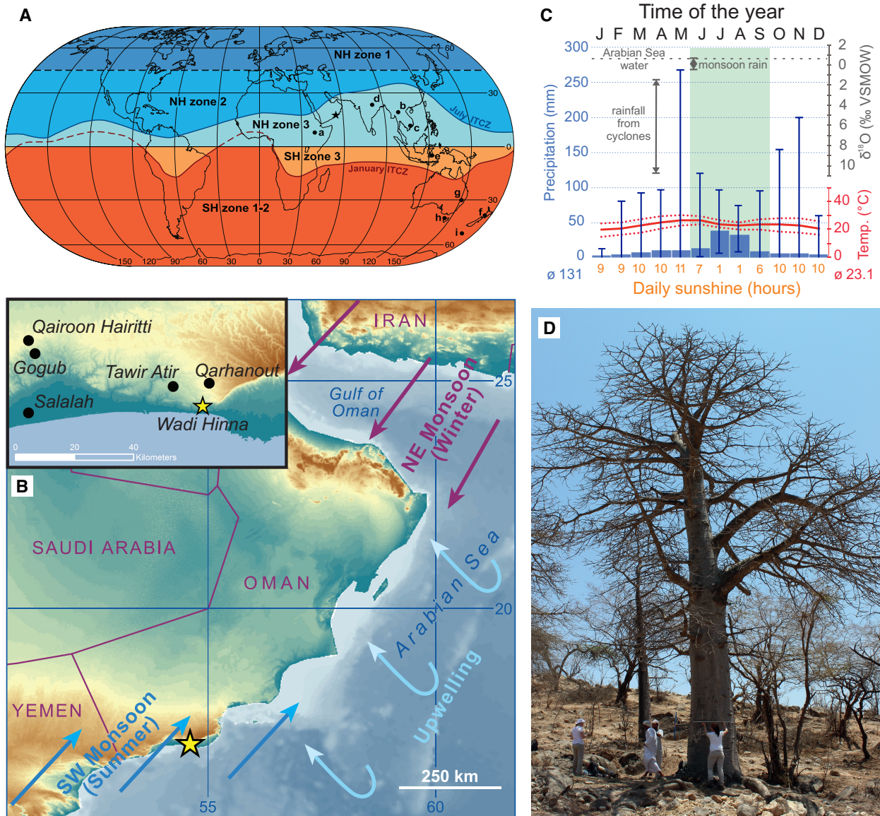
Figure 1: Context of the study site. (A) World map showing the northern hemispheric (NH) and southern hemispheric (SH) zones of atmospheric bomb ^{14}\text{C} (after Hua, et al. 2013). Zones close to the equator (NH3, SH3) are still underrepresented in studies reconstructing the atmospheric radiocarbon content. Star indicates study site; sites labeled with letters a-i correspond to sample locations of \text{F}^{14}\text{C} studies referred to in figure 5. (B) Map showing the location (yellow star) of the tree site Wadi Hinna (318 m asl) at the edge of the Dhofar mountains in southern Oman ( 17^{\circ} 03' \text{ N} , 54^{\circ} 36' \text{ E} ) (map topography based on SRTM and bathymetry data from Becker et al. 2009). Prevailing seasonal wind patterns are shown by blue (summer monsoon, rainfall season) and purple arrows (winter monsoon, dry season). Light blue arrows indicate upwelling of deep waters from the Arabian Sea. (C) Climate diagram for the area around Wadi Hinna ( 17.0\text{-}17.5^{\circ} \text{ N} , 54.0\text{-}54.5^{\circ} \text{ E} ) with average mean precipitation (bars indicating minima and maxima; source: GPCP, gpcp_V7_05) and temperature for 1942-2013 (dotted lines representing T min and T max , respectively; source: CRU TS4.01, GPCP V7_05). The isotopic signature of the Arabian Sea water and the precipitation around the study site is indicated in dark grey and varies significantly between monsoonal and non-monsoonal precipitation (Wushiki, 1991; Strauch et al., 2014). Average daily sunshine hours are given in orange (1979-1990, NOAA: ftp://ftp.atdd.noaa.gov/pub/GCOS/WMO-Normals/RA-II/OM/41316.TXT ) and the timing of the summer monsoon and the approximate growing season of the baobab trees is indicated in green. (D) Sampled baobab tree at Wadi Hinna.
