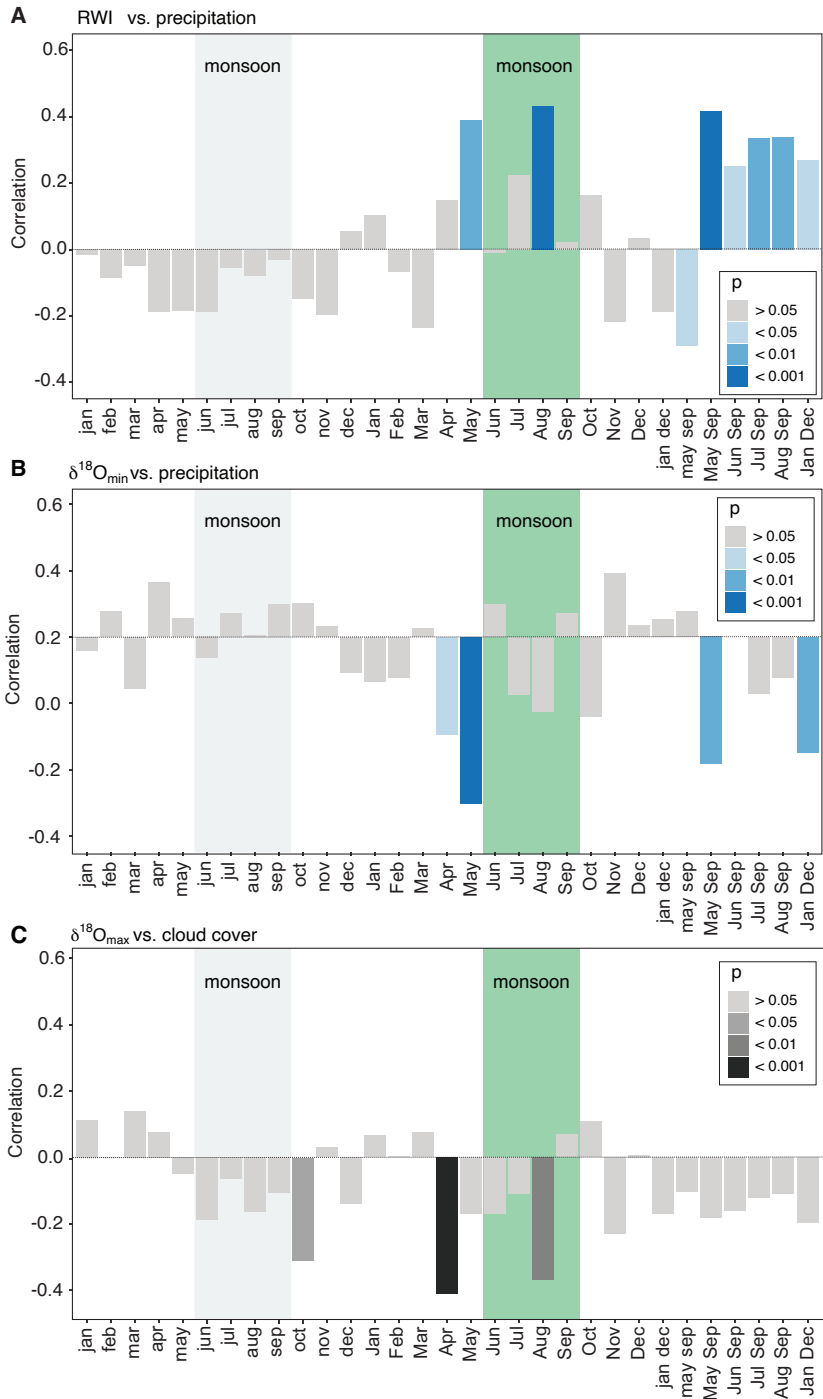
1045 Figure 7: Diagrams for the strongest correlations of baobab tree-ring parameters with monthly and seasonally resolved climate parameters. Months of the previous year are marked by lower case abbreviations, months of the current year by upper case abbreviations. The green box marks the average monsoon period. (A) Ring-width indices versus precipitation amount. (B) \delta^{18}\text{O}_{\text{min}} versus precipitation. (C) \delta^{18}\text{O}_{\text{max}} versus cloud cover. Apart from the actual monsoon season (Jun-Sep) also the pre-monsoon (Apr-May) has a significant influence on wood increment growth and \delta^{18}\text{O} isotope signature.
