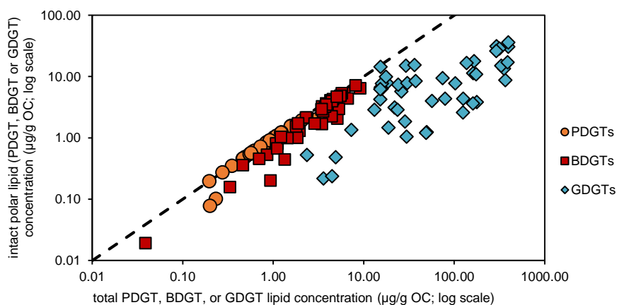
575 Figure 3: Intact polar lipid concentration against total lipid concentration (log scales) for each archaeal lipid type discussed in this study (PDGTs in orange, BDGTs in red and GDGTs in blue). The dashed line represents the 1:1 line.
