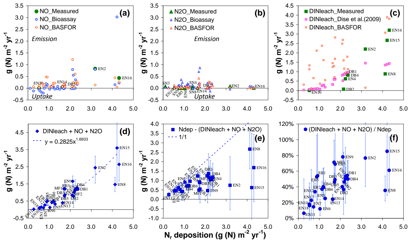
1660 Figure 3. Comparison of measured and estimated ecosystem inorganic N_r losses and their relationships to total atmospheric N_r deposition (x-axis) at the forest sites. NO fluxes (a) and N_2O fluxes (b) were either i) measured in situ using static or dynamic flux chambers, ii) scaled up from laboratory bioassay-derived T/WFPS relationships, or iii) simulated using the BASFOR ecosystem model (see text for details). DIN leaching (c) was either measured (lysimeter or suction cups), or predicted from the Dise et al. (2009) empirical algorithm. The sum of inorganic N_r losses (d) (DINleach + NO + N_2O ) was computed as the mean of measured values and modelled estimates. In panels (a)-(c), site names are indicated for sites where in situ measurements were available. 1665
