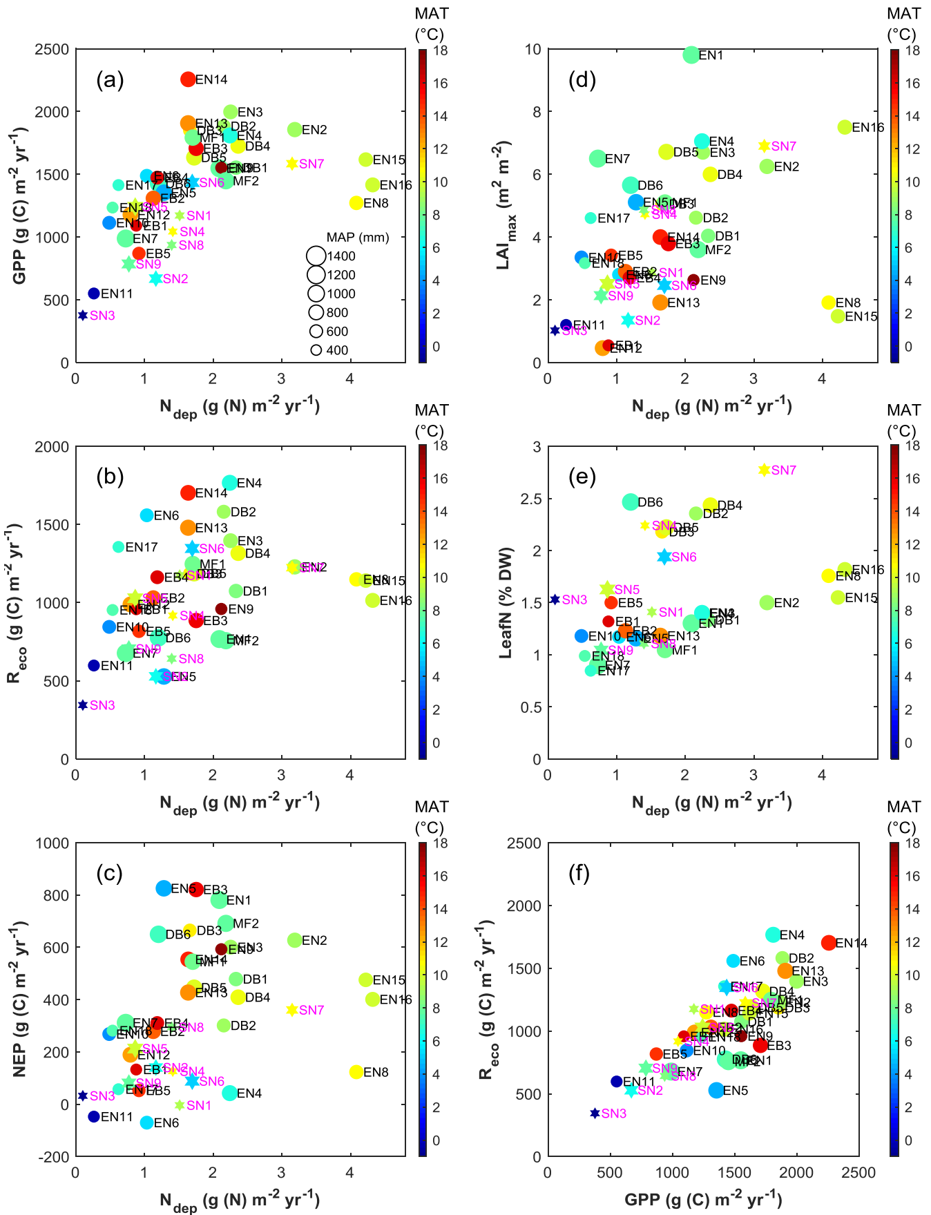
Figure 4. Overview of inter-annual mean EC-derived C flux estimates ( GPP, R_{\text{eco}} and NEP), ecosystem LAI and leaf N content, in relation to total (dry + wet) atmospheric N_r deposition (a-e), and relationship of R_{\text{eco}} to GPP (f), for forests (filled circles, black labels) and short semi-natural vegetation (filled stars, magenta labels). In all plots, the colour scale indicates mean annual temperature (MAT), while the symbol size is proportional to mean annual precipitation (MAP, scale provided in panel a).
