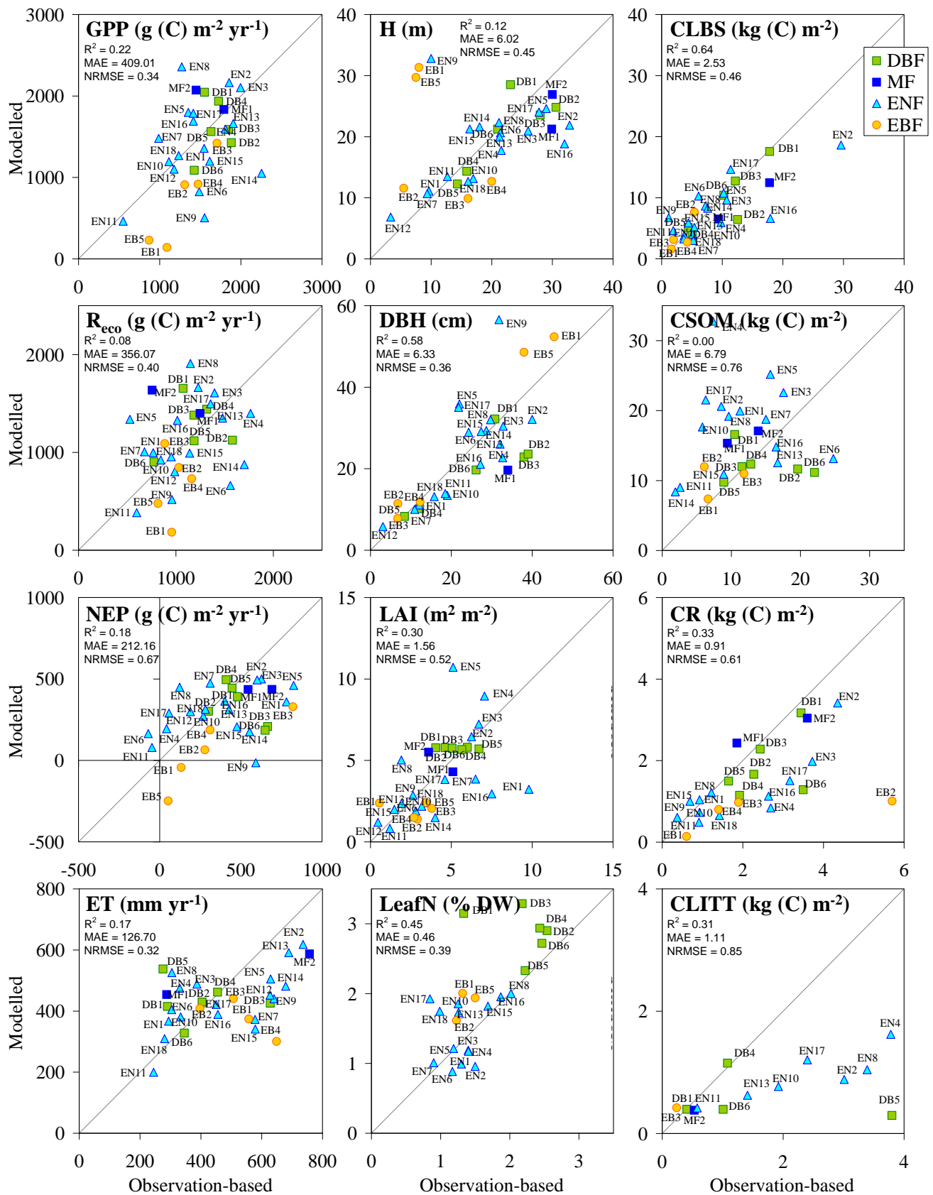
1680 Figure 6. BASFOR baseline simulations for all forest sites; model outputs and observation-based values were averaged over the years between the first and last available observations. Note that model simulations include MF and EBF sites, for which the model was not calibrated in Cameron et al. (2018); the two MF runs were made using the parameter table for DBF, while the five EBF runs were made using the parameter table for ENF to allow continued growth throughout the year. H: mean tree height; DBH: mean diameter at breast height; CLBS, CSOM, CR, CLITT: carbon stocks in leaves, branches and stems, in soil organic matter, in roots, and in litter layers, respectively; MAE: mean absolute error; NRMSE: root mean square error normalised to the mean.
