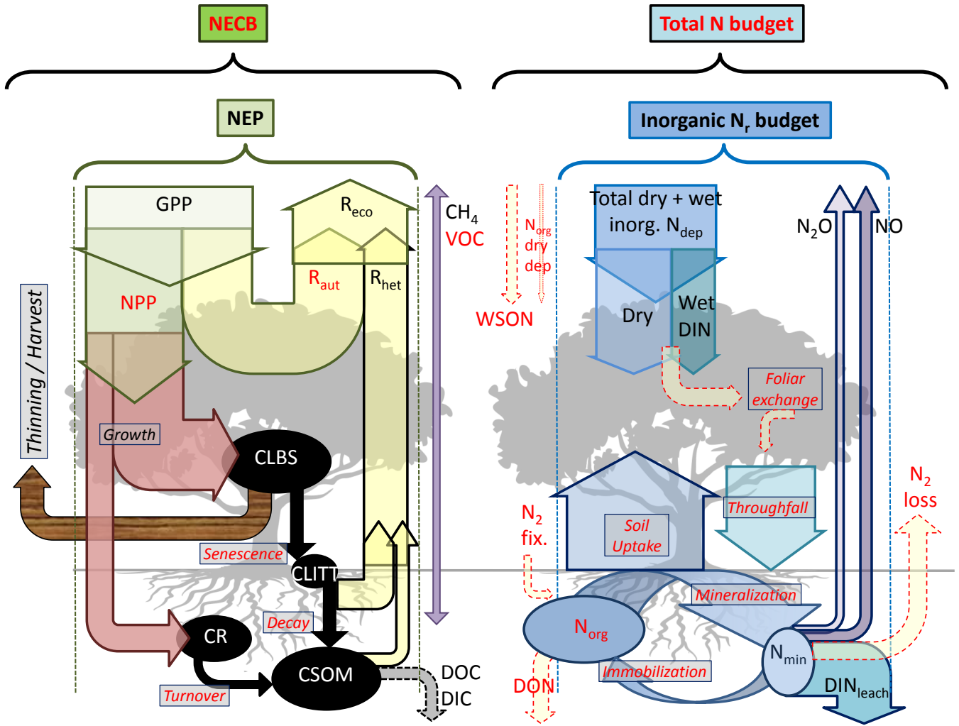
Figure 1. Flux terms and boundaries of the carbon (left) and nitrogen (right) budgets discussed in this paper. Net ecosystem productivity NEP = GPP - R_{eco} ( \approx NPP - R_{het} ) based on multi-annual eddy covariance CO_2 flux data. The net ecosystem carbon balance (NECB) includes in addition other C loss fluxes such as DIC/DOC, CH_4 and VOC, as well as harvest, thinning or other disturbances (e.g. fire). Inorganic reactive nitrogen ( N_r ) budget = N_{dep} - DIN_{leach} - NO - N_2O . The total N budget includes in addition organic nitrogen deposition (WSON) and leaching (DON), as well as N_2 inputs and losses from biological fixation and denitrification, respectively. CLBS, CSOM, CR, CLITT: carbon stocks in leaves, branches and stems, in soil organic matter, in roots, and in litter layers, respectively. Terms highlighted in red indicate that direct or measurement-based estimates were not available for some or all sites in our datasets (see also Table 2 for a list of acronyms, Table 3 for a summary of methods, and Table S6 for data availability).
