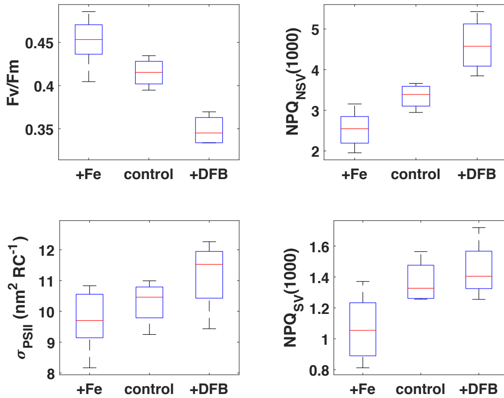
895 Figure 2: FRRf results after ~53 hours for the 3 pooled incubation experiments. The respective treatments are indicated on the x- axes (2 nM and 0.2 nM Fe additions were pooled into +Fe), and measured parameters are on the y-axes. NPQ capacity was estimated at 1000 \mu\text{mol quanta m}^{-2} \text{s}^{-1} after 24-minute exposure to increasing actinic light intensities (see Fig. S2 for details of the fluorescence light curves). Boxplots show the sample medians in red, with the blue boxes indicating the 25 th and 75 th percentiles; whiskers extend to the most extreme data points. All +Fe treatments were significantly different from the respective DFB treatments (Wilcoxon rank sum test, p < 0.05 ), and except for \sigma_{PSII} , all +Fe treatments were also significantly different from the respective control treatments.
