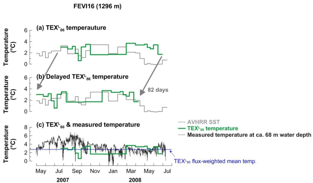
Figure 7. Changes in TEX 86 L -derived temperatures and satellite-derived SSTs (a), time-delayed TEX 86 L temperatures (b), sensor measured temperatures at approximately 68 m water depth at site FEVI16.
