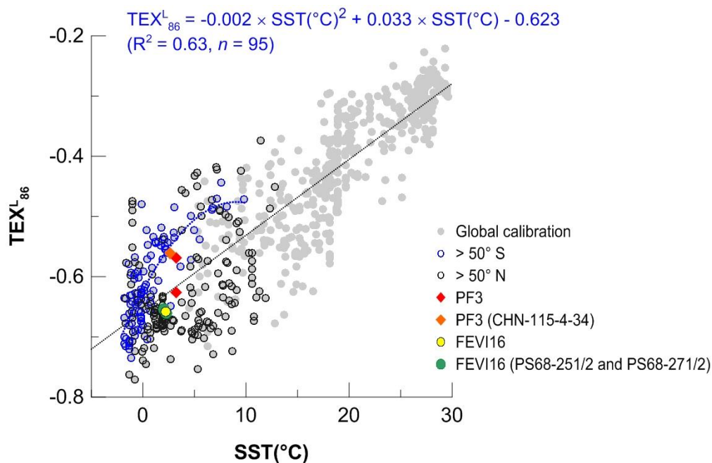
Figure 9. Correlation of TEX 86 L values with mean annual SSTs in the global ocean (gray symbols; Tierney and Tingley, (2015) and reference therein). Blue and black round symbols represent the high latitude regions higher than 50° S and 50° N, respectively. In the southern regions (>50° S), TEX 86 L values have a polynomial correlation with maSSTs ( R^2 = 0.63 , n = 95 ). Red and orange diamonds represent the flux-weighted mean TEX 86 L of the two traps at the site PF3 and TEX 86 L on the surface sediment (CHN-115-4-34), respectively. Yellow and green round symbols represent the flux-weighted mean TEX 86 L at the site FEVI16 and TEX 86 L on the surface sediments (PS68-251/2 and PS68-271/2), respectively.
