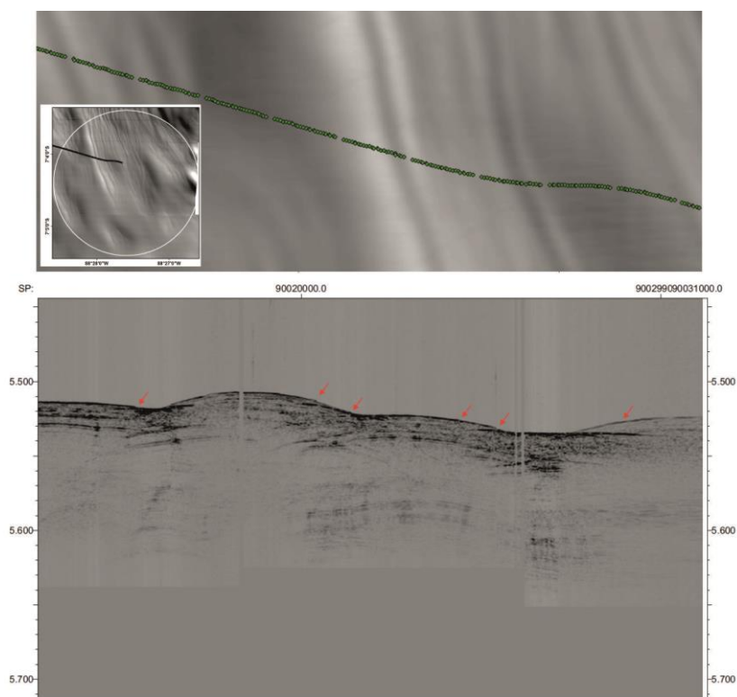
Figure 1: Section of a sub-bottom profile (below) crossing some of the channel structures within the DEA (above). Red arrows indicate the crossing of such a structure.
