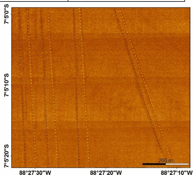
790 Figure G1: The plough marks visible in the SSS map show the offset of the SSS data before (yellow dotted) and after (black dotted) geo-referencing based on the MB data sets. An offset of approximately 30-50 m, in some areas also up to 80 m can be detected.
