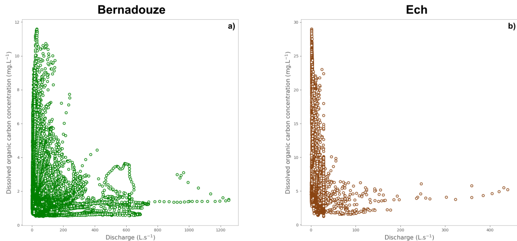
Fig. 1. DOC concentration vs Q plots
