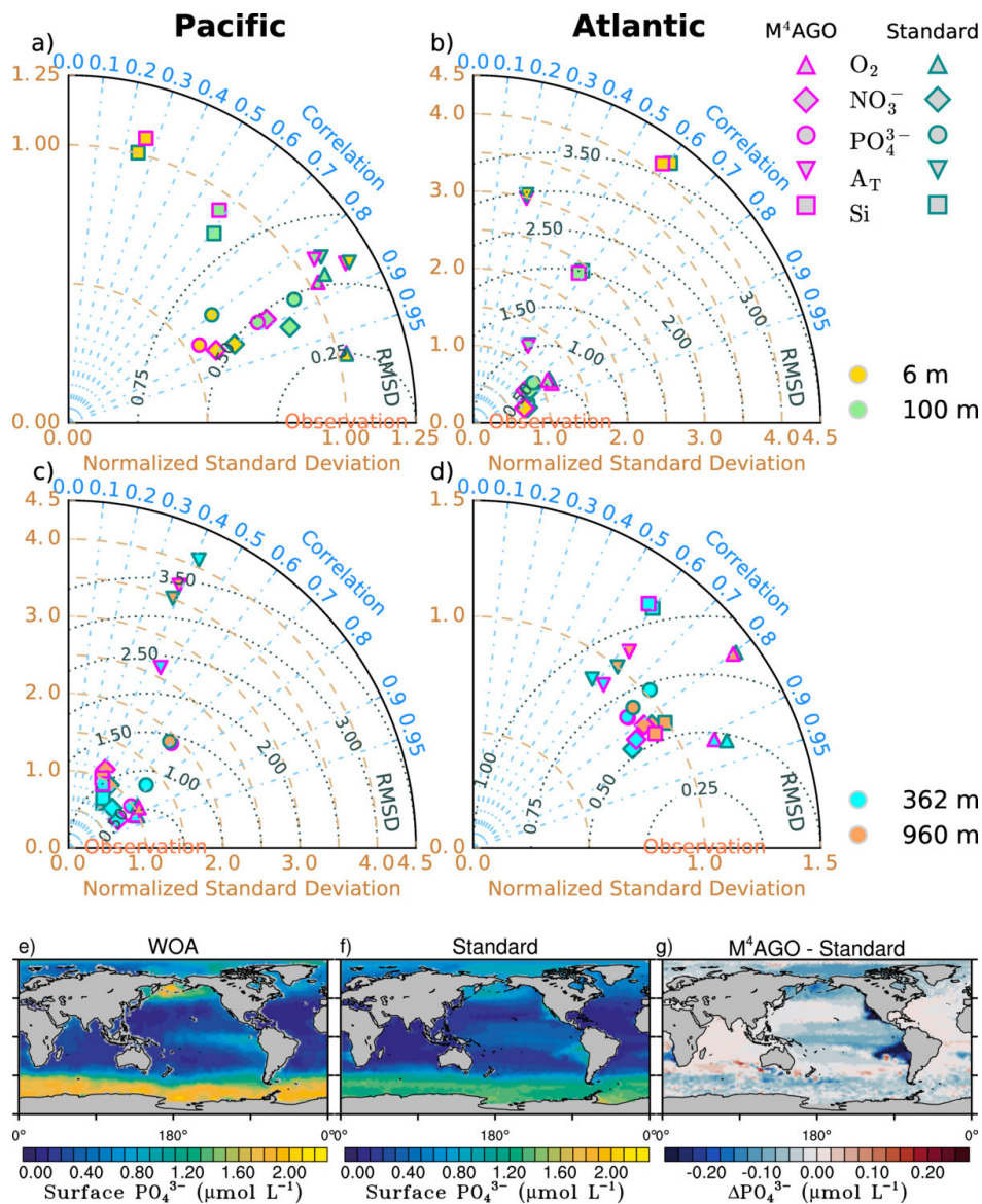
Figure 13. a-d) Taylor diagram for tracers (oxygen, O 2 , nitrate, NO 3 - , phosphate, PO 4 3- , silicate, Si) in comparison to the World Ocean Atlas data (Boyer et al., 2013; Garcia et al., 2014b) and, in the case of total alkalinity, A T , to GLODAPv2 data (Lauvset et al., 2016). a) and c): Pacific, b) and d) Atlantic for upper panel 6 m and 100 m. Lower panel 362 m and 960 m. e) surface phosphate concentration in WOA f) in the standard run and g) difference plot between M 4 AGO and the standard run.
