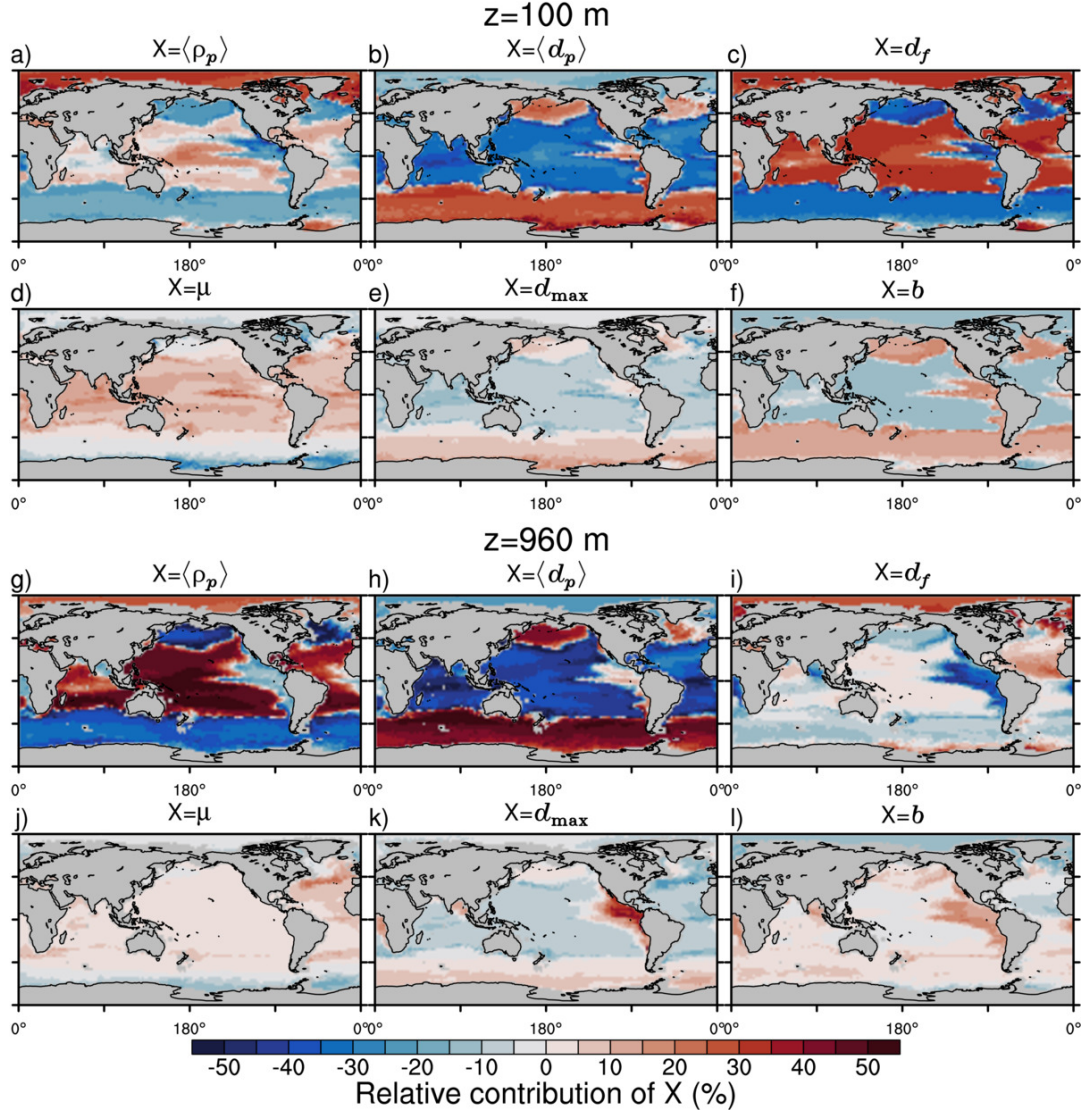
Figure 10. Qualitative first order relative contributions of marine aggregate properties to the change of local mean sinking velocity compared to a global mean aggregate spectrum at depth z . a)-f): 100 m, g)-l) 960 m. Mathematical symbols are: \langle \rho_p \rangle : mean primary particle density; \langle d_p \rangle : mean primary particle diameter; d_f : fractal dimension; \mu : dynamic molecular viscosity; d_{\max} : maximum aggregate diameter; b : aggregate number distribution slope.
