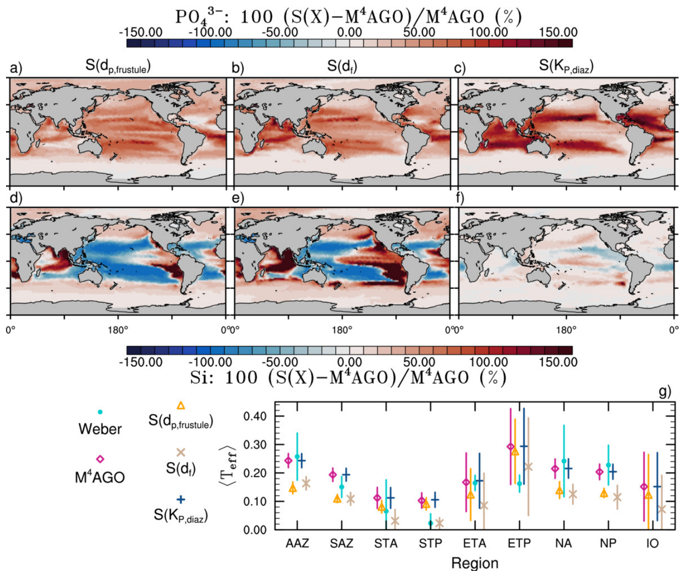
Figure 15. Sensitivity of a)-c) surface phosphate, d)-f) silicate concentrations, and g) POC transfer efficiency to diatom frustule size, d_{p,\text{frustule}} ( S(d_{p,\text{frustule}}) ), modified from 20\mu\text{m} to 10\mu\text{m} ), the half-saturation constant for phosphate uptake by diazotrophs ( S(K_{P,\text{diaz}}) ), modified from 0.05\mu\text{mol L}^{-1} to 0.1\mu\text{mol L}^{-1} ), and fractal dimension, d_f ( S(d_f) ), from variable to constant d_f = 2 ). Error bars in g) represent regional standard deviation and for Weber et al. the uncertainty for the reconstruction of the regional transfer efficiency.
