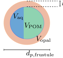
Figure 2. Diatom frustule and the remineralization state-dependent composition of the void. l denotes the thickness of the opal shell with volume V_{opal} . V_{aq} and V_{POM} are the encapsulated volumes of water and POM, respectively. d_{p,frustule} is the diameter of the diatom frustule.
