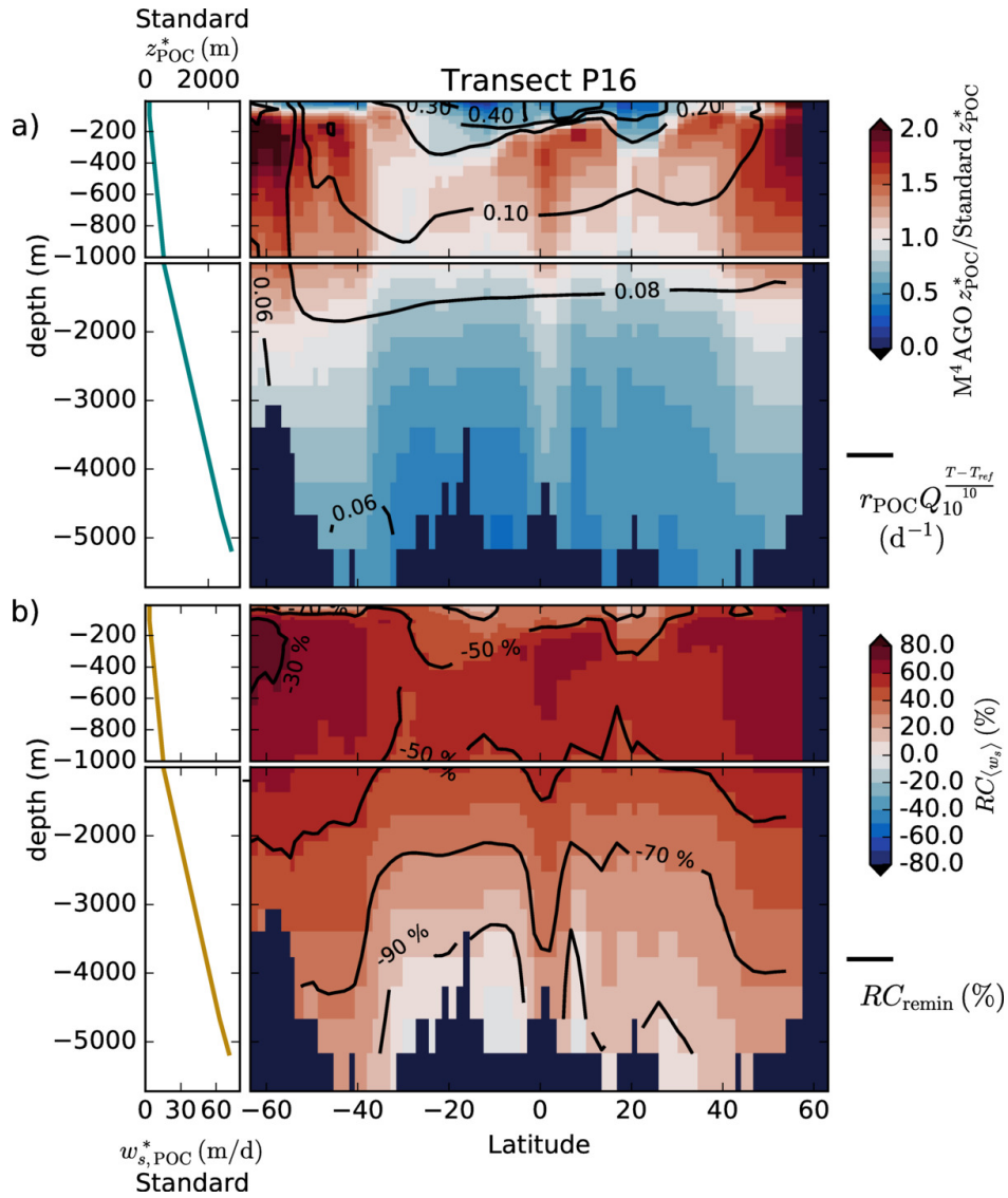
Figure 9. a) Remineralization length scale ratio of M^4AGO to the standard model version at the World Ocean Atlas transect P16. We here focus on showcasing the temperature effect on remineralization and calculated the remineralization length scales, z_{POC}^* , without oxygen limitation of remineralization which cancels out for equal O_2 concentrations. Values smaller than one imply stronger POC flux attenuation in M^4AGO than in the standard run. For reference, the RLS in the standard run is given at top left. The standard RLS is increasing due to increasing sinking velocity, w_{s,POC}^* , with depth (shown bottom left). Contour lines provide the Q_{10} factor temperature-dependent remineralization rates with r_{POC} at reference temperature T_{ref} in M^4AGO . In the standard run, the aerobic rate is globally constant ( 0.026 d^{-1} ). b) Relative contributions of sinking, RC_{(w_s)} , and remineralization, RC_{remin} , to difference between standard and M^4AGO run. Contour lines provide the relative contribution of remineralization.
