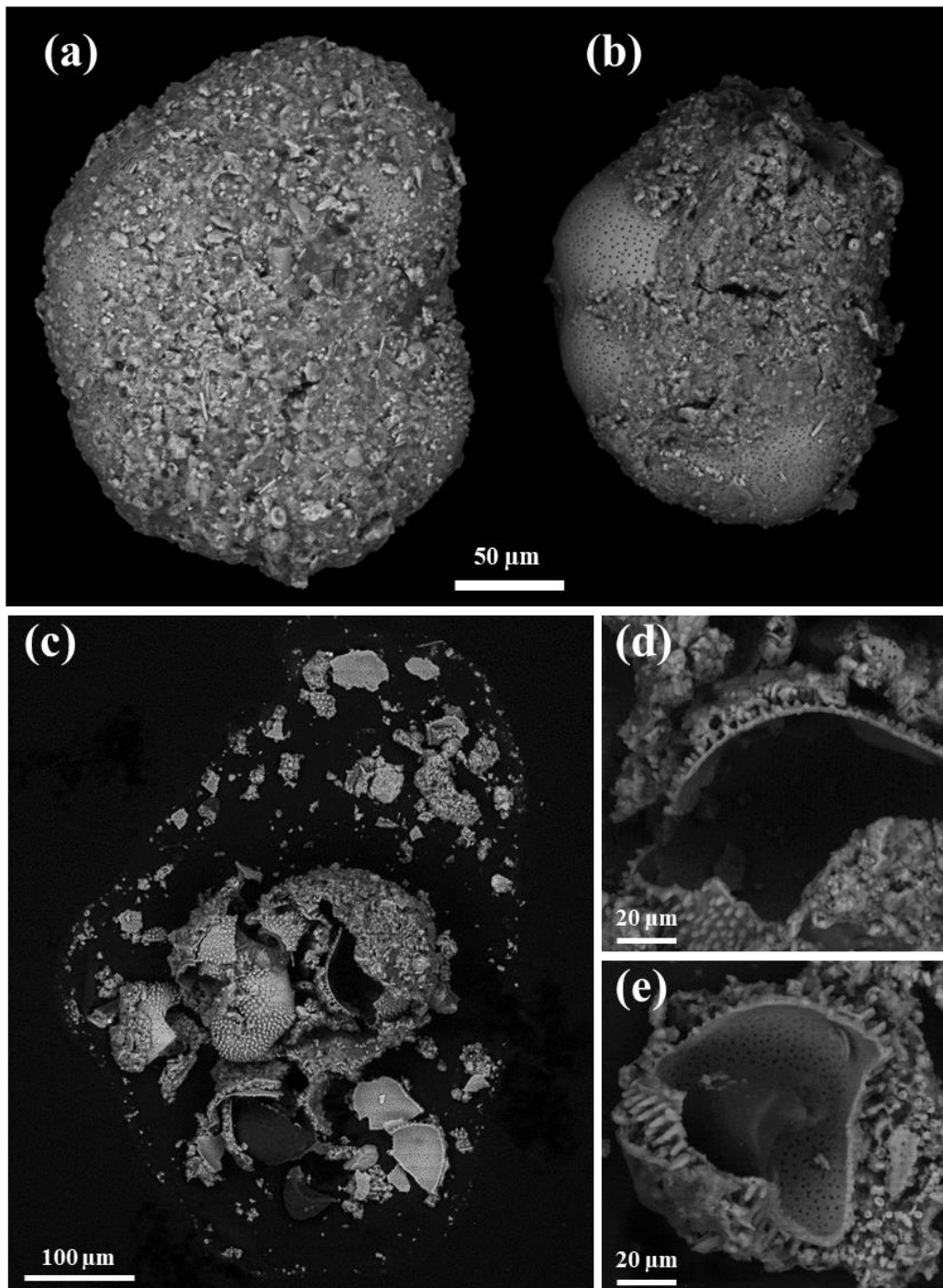
Figure 2: SEM images of (a) fully encrusted specimen, (b) partially encrusted specimen, (c) crushed encrusted specimen of Elphidium magellanicum . Note the thinness of the crust and the spinose structures on (d) and (e).
