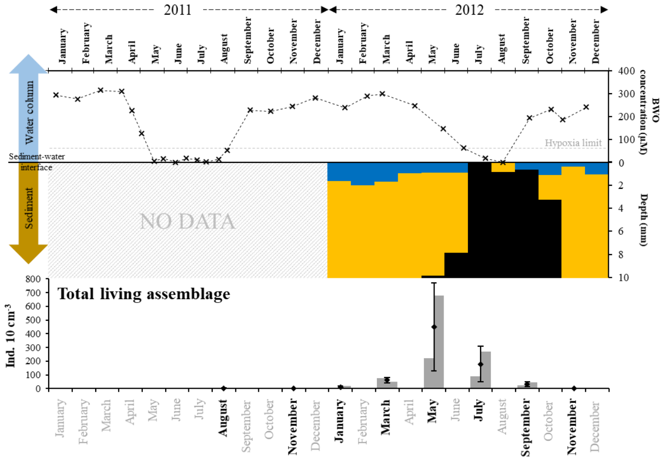
830 Figure 8: The top panel represents bottom-water oxygen concentrations ( \mu\text{mol L}^{-1} ) in 2011 and 2012 at station 1, from Donders et al. (2012) and Seitaj et al. (2017). The grey horizontal dotted line indicates the hypoxia limit ( 63 \mu\text{mol L}^{-1} ). The middle panel represents the depth (in mm) distribution of the oxic (blue), absence of oxygen and sulphides (orange,) and sulphidic (black) zones within the sediment in 2012, from Seitaj et al. (2015). The bottom panel shows the total living foraminiferal abundances for both replicates (grey bars), mean abundances (diamonds) and standard deviations (black error bars) calculated for the two replicates, 835 for all investigated months (in bold) in 2011 and 2012.
