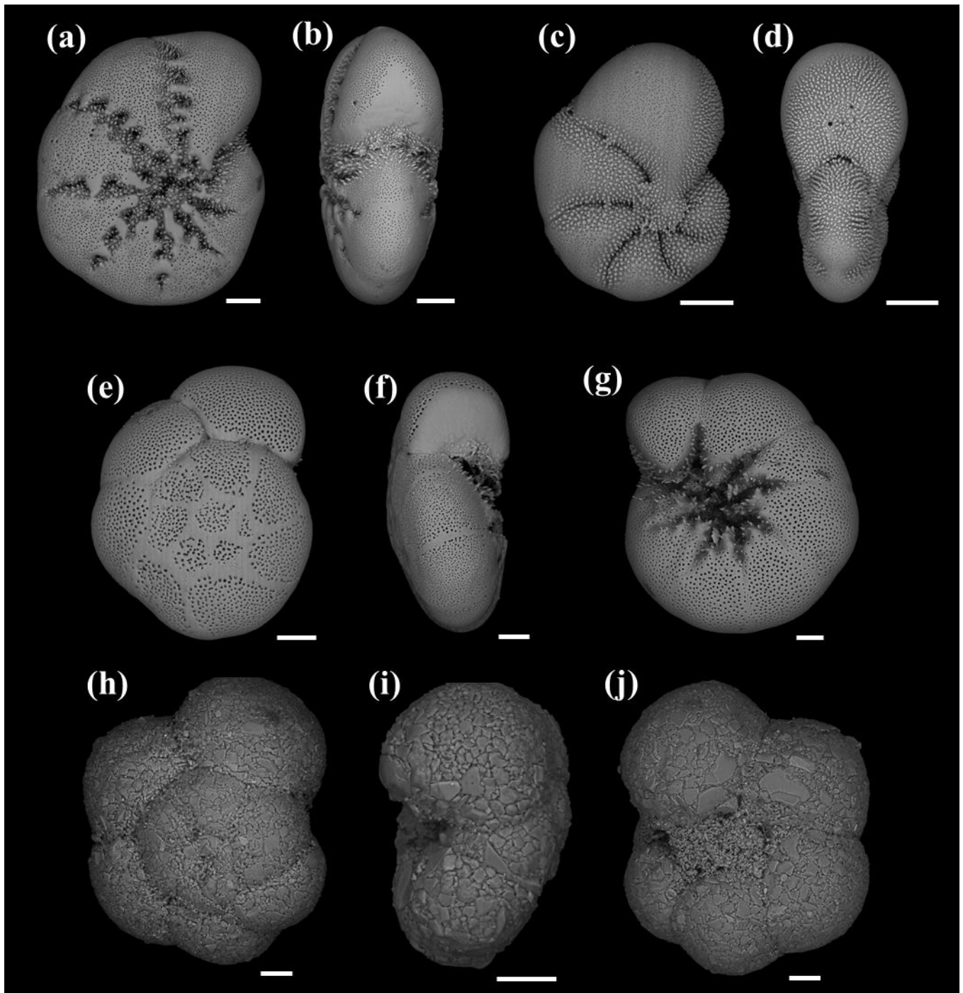
810 Figure 4: SEM images of Elphidium selseyense in lateral (a) and peripheral (b) view, Elphidium magellanicum in lateral (c) and peripheral (d) view, Ammonia sp. T6 in spiral (e), peripheral (f) and umbilical (g) view, and Trochammina inflata in spiral (h), peripheral (i) and umbilical (j) view. All scale bars are 50 µm.
