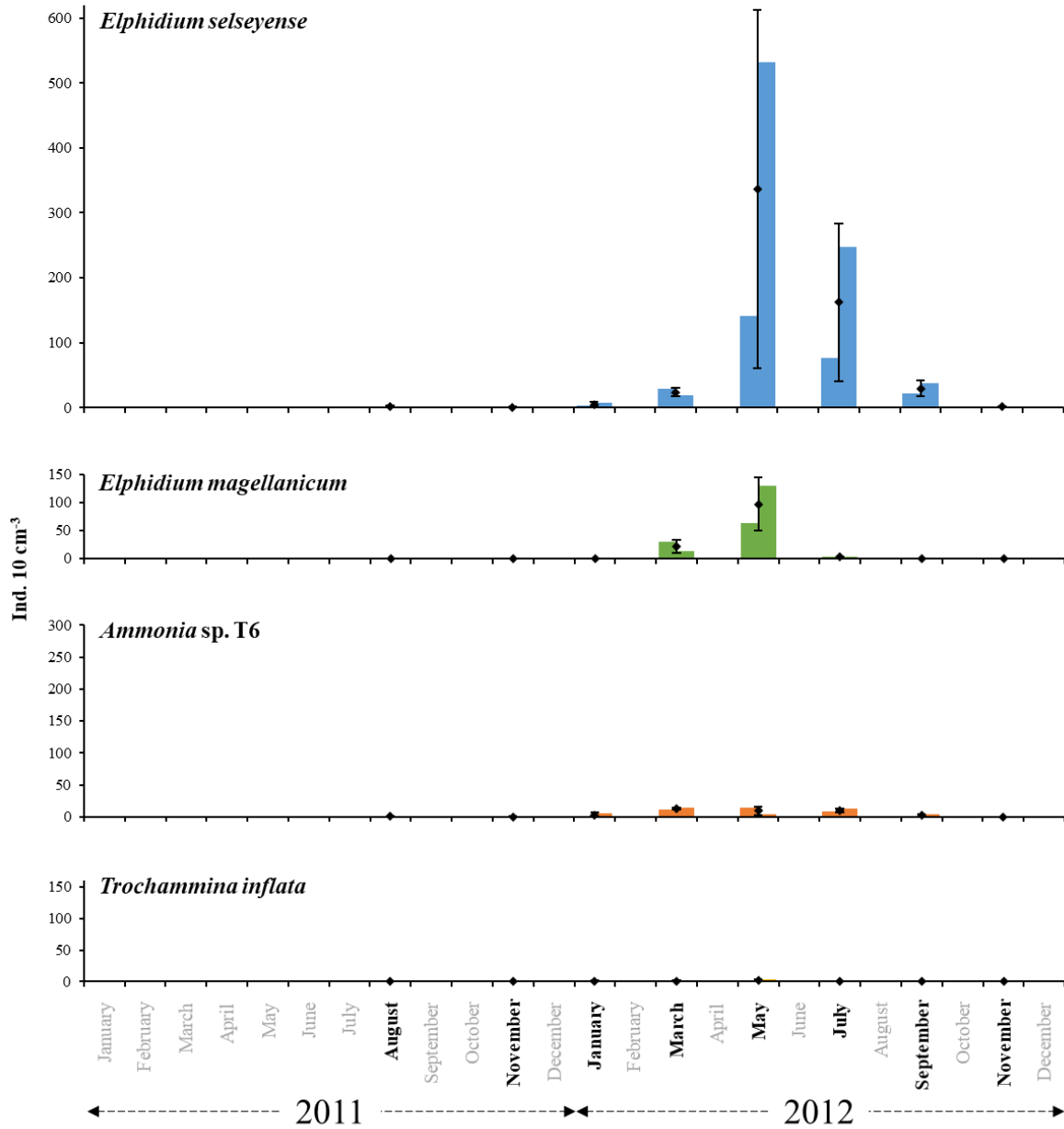
815 Figure 5: The bars represent the living foraminiferal abundances for the two replicates for Elphidium selseyense (blue), Elphidium magellanicum (green), Ammonia sp. T6 (orange) and Trochammmina inflata (yellow) at station 1 in 2011 and 2012. The mean abundances (diamonds) and standard deviations (black error bars) were calculated for the two replicates. All abundances values are for 0–1cm layer and were standardised to 10 cm 3 . Months where foraminiferal communities were investigated are indicated in bold. Scales were chosen in order to facilitate comparison with station 2.
