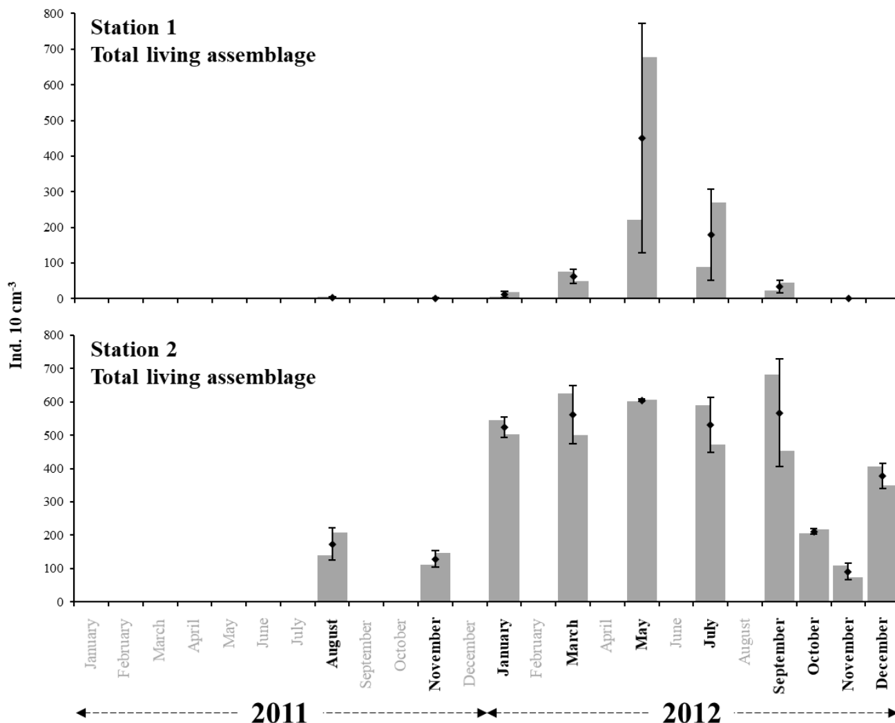
805 Figure 3: The grey bars represent the living foraminiferal abundances for the two replicates. The mean abundances (diamonds) and standard deviations (black error bars) were calculated for the two replicates for stations 1 (34 m depth, top panel) and 2 (23 m depth, bottom panel). All abundance values are for the 0–1 cm layer and were standardised to 10 cm 3 . Months where foraminiferal communities were investigated are indicated in bold (excluding October and December at station 1).
