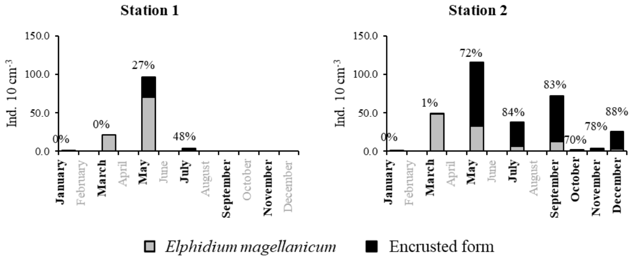
Figure 7: Mean abundances (ind. 10 cm -3 ) of non-encrusted (grey) and encrusted forms (black) of Elphidium magellanicum in 2012, at station, 1 (left) and 2 (right), with proportion of encrusted forms above each bar (in %). Investigated months are indicated in bold.
