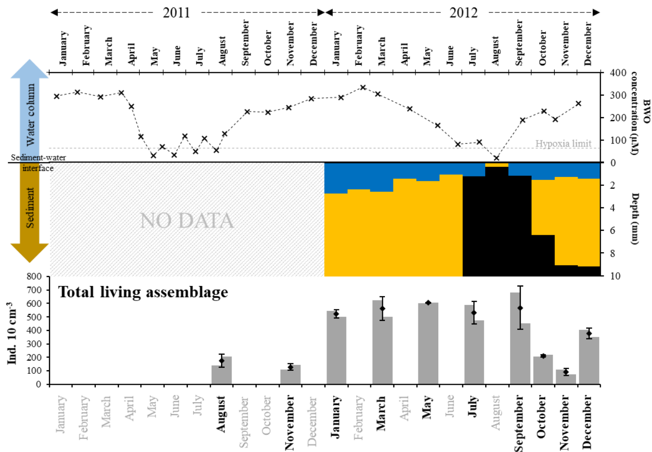
Figure 9: The top panel represents bottom-water oxygen concentrations ( \mu\text{mol L}^{-1} ) in 2011 and 2012 at station 2, from Donders et al. (2012) and Seitaj et al. (2017). The grey horizontal dotted line indicates the hypoxia limit ( 63 \mu\text{mol L}^{-1} ). The middle panel represents the depth (in mm) distribution of the oxic (blue), suboxic (orange, absence of oxygen and sulphides) and sulphidic (black) zones within the sediment in 2012. The bottom panel shows the total living foraminiferal abundances for both replicates (grey bars), mean abundances (diamonds) and standard deviations (black error bars) calculated for the two replicates, for all investigated months (in bold) in 2011 and 2012.
