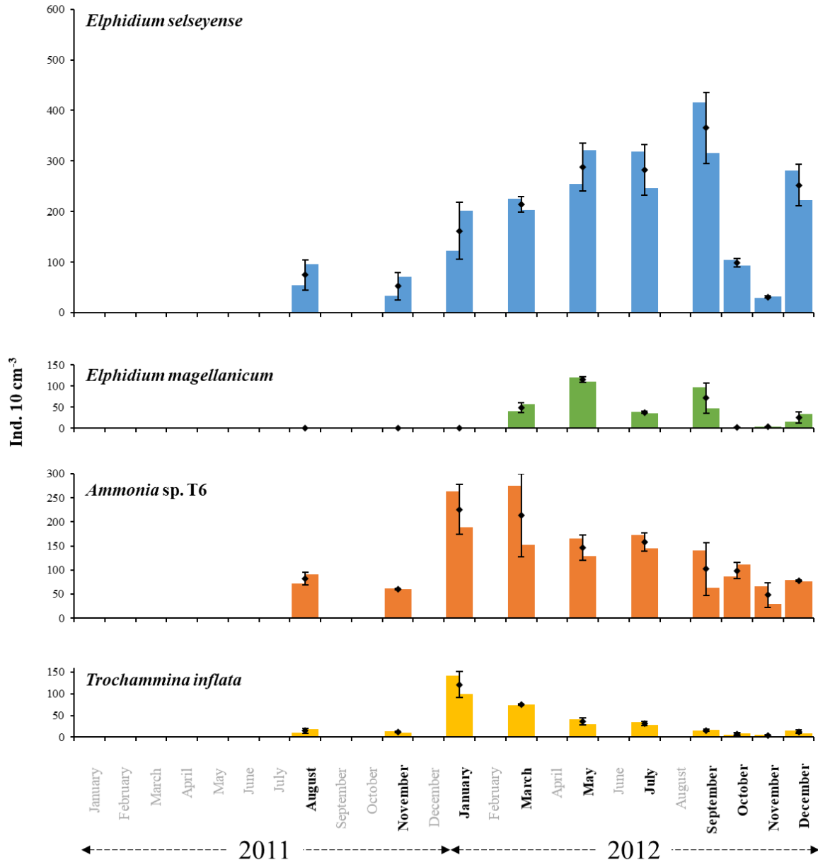
820 Figure 6: The bars represent the living foraminiferal abundances for the two replicates for Elphidium selseyense (blue), Elphidium magellanicum (green), Ammonia sp. T6 (orange) and Trochammina inflata (yellow) at station 2 in 2011 and 2012. The mean abundances (diamonds) and standard deviations (black error bars) were calculated for the two replicates. All abundances values are for 0–1cm layer and were standardised to 10 cm 3 . Months where foraminiferal communities were investigated are indicated in bold. Scales were chosen in order to facilitate comparison with station 1.
