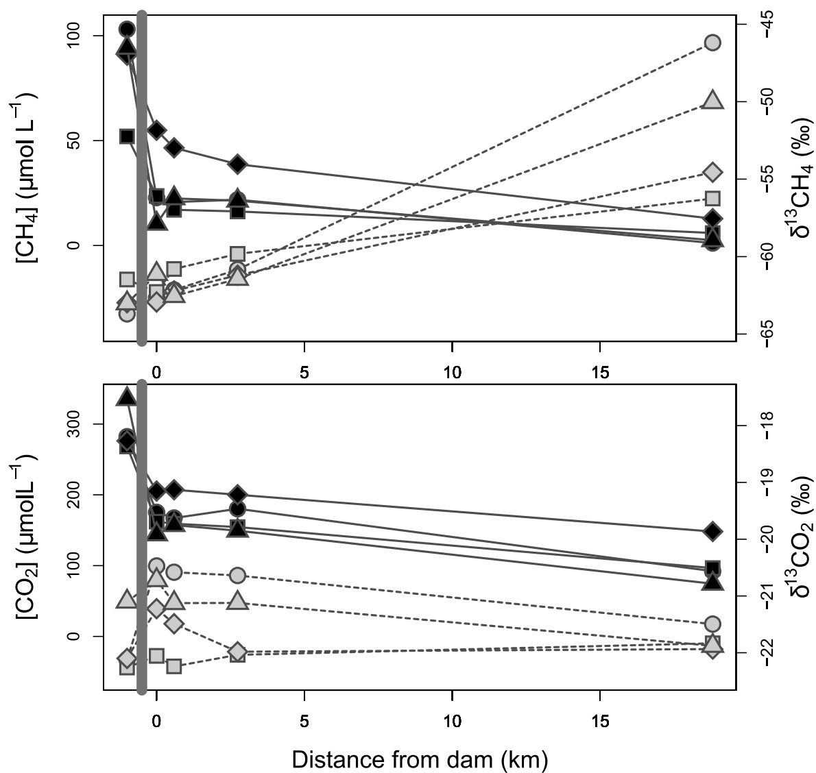
570 Figure 3: Concentrations (black symbols and solid line) and \delta^{13}\text{C} (gray symbols and dotted lines) of \text{CO}_2 and \text{CH}_4 from right upstream of the dam (gray band) to 19 km downstream in the outflow river. Circles, squares, diamonds, and triangles represent values from Nov-Dec 2016, Apr-May 2017, Feb-Mar 2018, and Aug 2018 respectively.
