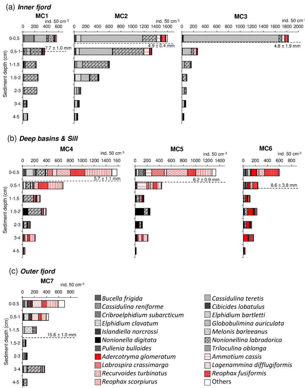
Figure 4: Foraminiferal vertical distribution from 0 down to 5 cm sediment depth (>150 µm fraction) for a) the inner fjord (stations MC1 to MC3) b) deep basins (stations MC4 and MC5) and sill (station MC6) and c) outer fjord (station MC7). Calcareous species are shown using different grey textures, whereas agglutinated species using different red textures. The dashed black line represents the average oxygen penetration depth (OPD) at each station.
