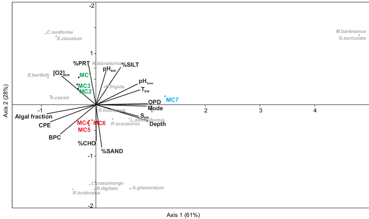
Figure 5: Canonical Correspondence Analysis based on real abundances (ind. 50 cm -2 ) of the living faunas in the 0-5 cm sediment layer (> 150 µm size fraction) considering the major species (> 5%) vs environmental variables described in tables 1, S2, S3.
