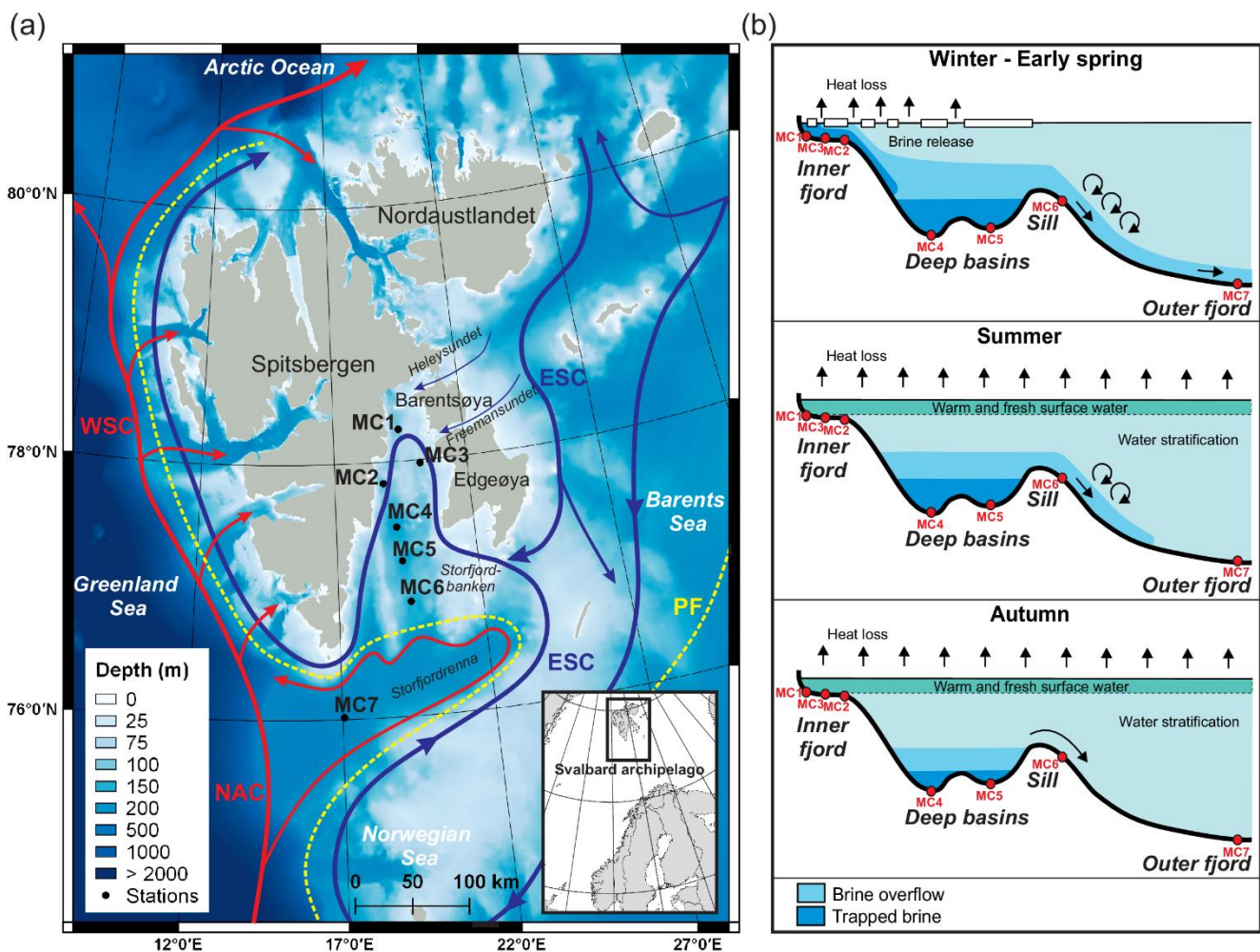
Figure 1: a) Bathymetric map showing the main currents circulation around the Svalbard archipelago (currents from Skogseth et al., 2005b and Misund et al., 2016) and location of the sampling stations. The red lines represent the warm North Atlantic waters carried by the Norwegian Atlantic Current (NAC) and West Spitsbergen Current (WSC). The blue lines represent the cold Arctic waters carried by the East Spitsbergen Current (ESC). Dotted yellow line represents the Polar front (PF). Bathymetry obtained from EMODnet ( http://portal.emodnet-bathymetry.eu ) and map elaborated with QGIS (made with Natural Earth). b) Longitudinal bathymetric profile sketches showing seasonal formation and flow of brines in the inner and outer Storfjorden (modified from Skogseth et al., 2005a and Rasmussen and Thomsen, 2015) and indicative location of the sampling stations (red dots).
