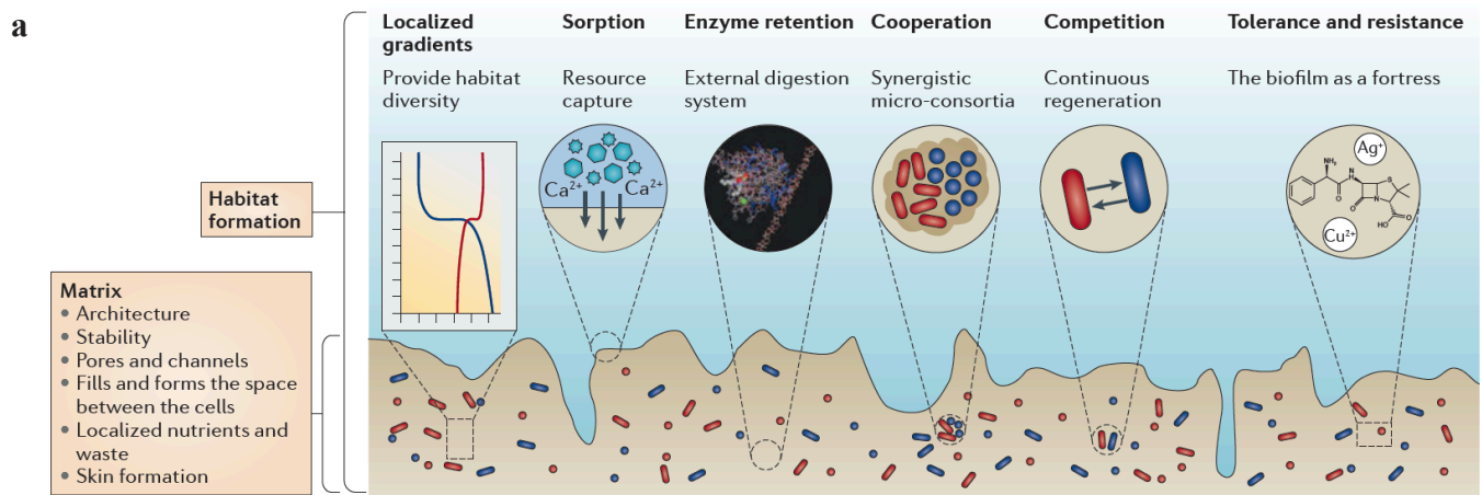
Fig. 1. (a) Schematic diagram showing biofilm structure and function, and the biological and chemical processes that biofilms influence. (b) Extracellular polymeric substance (EPS) halos and their possible influence on interactions between hypha and mineral surfaces (based on observations by Gazzè et al., 2013). ( Fig. 1a reproduced with permission; Flemming et al.: Nat. Rev. Microbiol. , 14, 563-575, 2016.)
