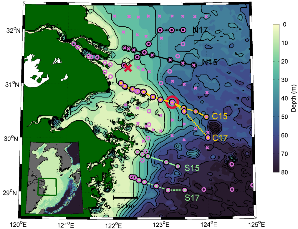
825 Figure 1. Map of the study area off the Changjiang Estuary. Crosses represent CTD cast stations conducted on 27 August–5 September in 2015 and circles show CTD cast stations on 24–29 July in 2017. Lines represent northern sections (N15 in 2015 and N17 in 2017), central sections (C15 in 2015 and C17 in 2017), and southern sections (S15 in 2015 and S17 in 2017). Larger circle represents the mooring M1 location. The larger cross shows the location, where wind data were gathered. The color scale shows depth (m) of the study area. The inlay shows the study area in the East China Sea.
