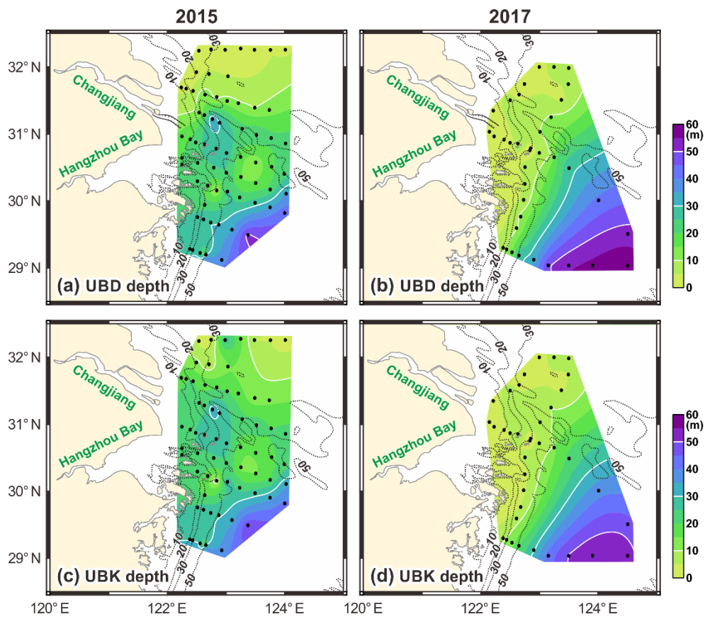
865 Fig. 7. Maps of AOU isoline 2 mg l -1 (upper boundary of the DO depletion, UBD) depth (upper panels) and temperature isoline 24.5 °C (upper boundary of KSSW, UBK) depth (lower panels) in 2015 (left panels) and in 2017 (right panels).
