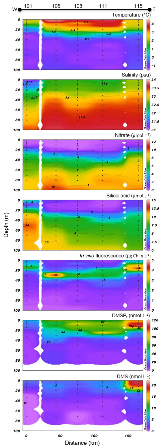
Figure 7: North Water (NOW) cross section of the vertical distributions of temperature, salinity, nitrate, silicic acid, in vivo fluorescence, DMSP 1 and DMS.
