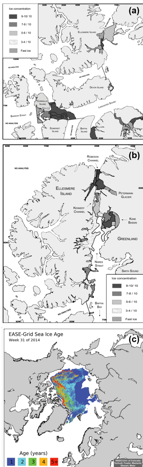
Figure 2: Ice charts adapted from the Canadian Ice Services (CIS) of Environment Canada showing the presence of ice edges in (a) Lancaster Sound with 9-10/10 ice concentrations (> 15 cm) extending from Devon Island into the Prince Regent Inlet between Somerset and Baffin islands (July 22, 2014); and in (b) Nares Strait with 9-10/10 ice concentrations near Petermann Glacier (August 1, 2014); Pannel (c) shows the presence of MYI (2 to 5+ years) at the entrance of Robeson Channel as well as a band of FYI (1) (Ease-Grid Sea Ice Age, Version 3 data set, Tschudi et al. (2016)). See the Canadian Ice Services Archives website for more details about sea ice characteristics. Note that Nares Strait includes Smith Sound, Kane Basin, Kennedy Channel, Hall Basin and Robeson Channel.
