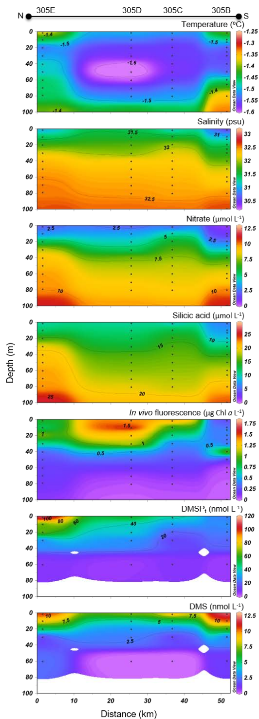
Figure 4: Barrow Strait (BS) cross section of the vertical distributions of temperature, salinity, nitrate, silicic acid, in vivo fluorescence, DMSP f and DMS.
