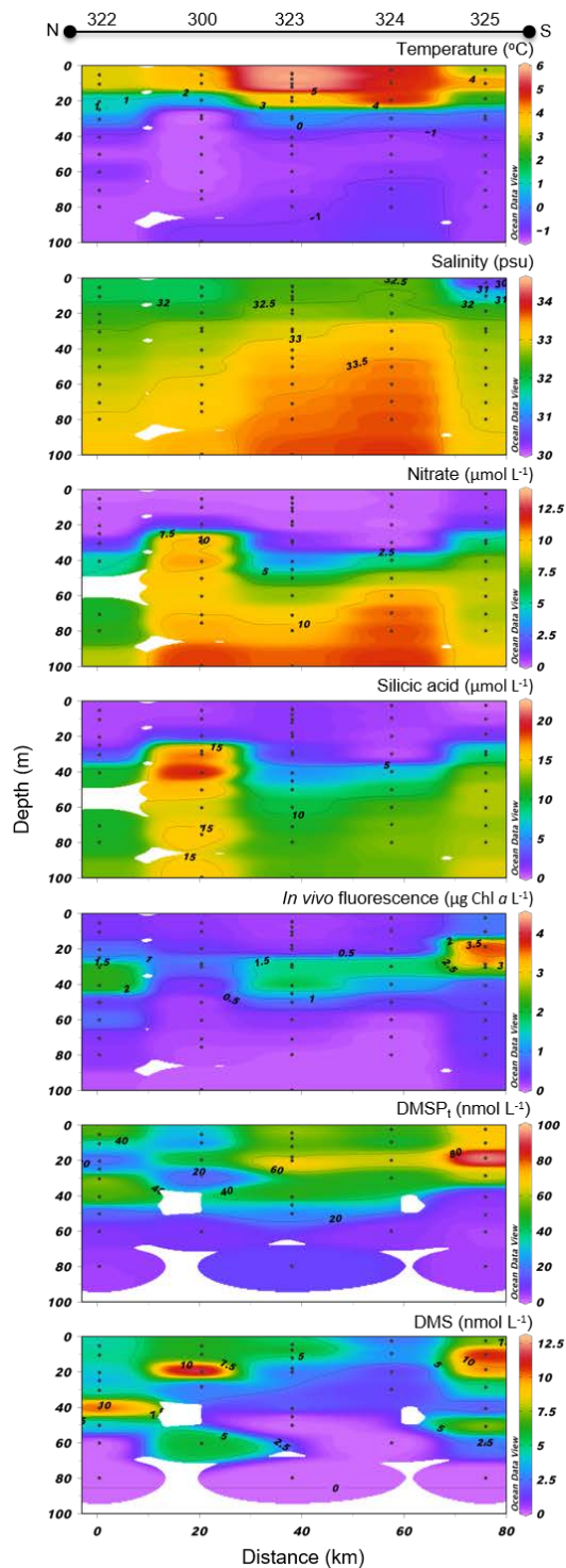
Figure 5: Lancaster Sound (LS) cross section of the vertical distributions of temperature, salinity, nitrate, silicic acid, in vivo fluorescence, DMSP 1 and DMS.
