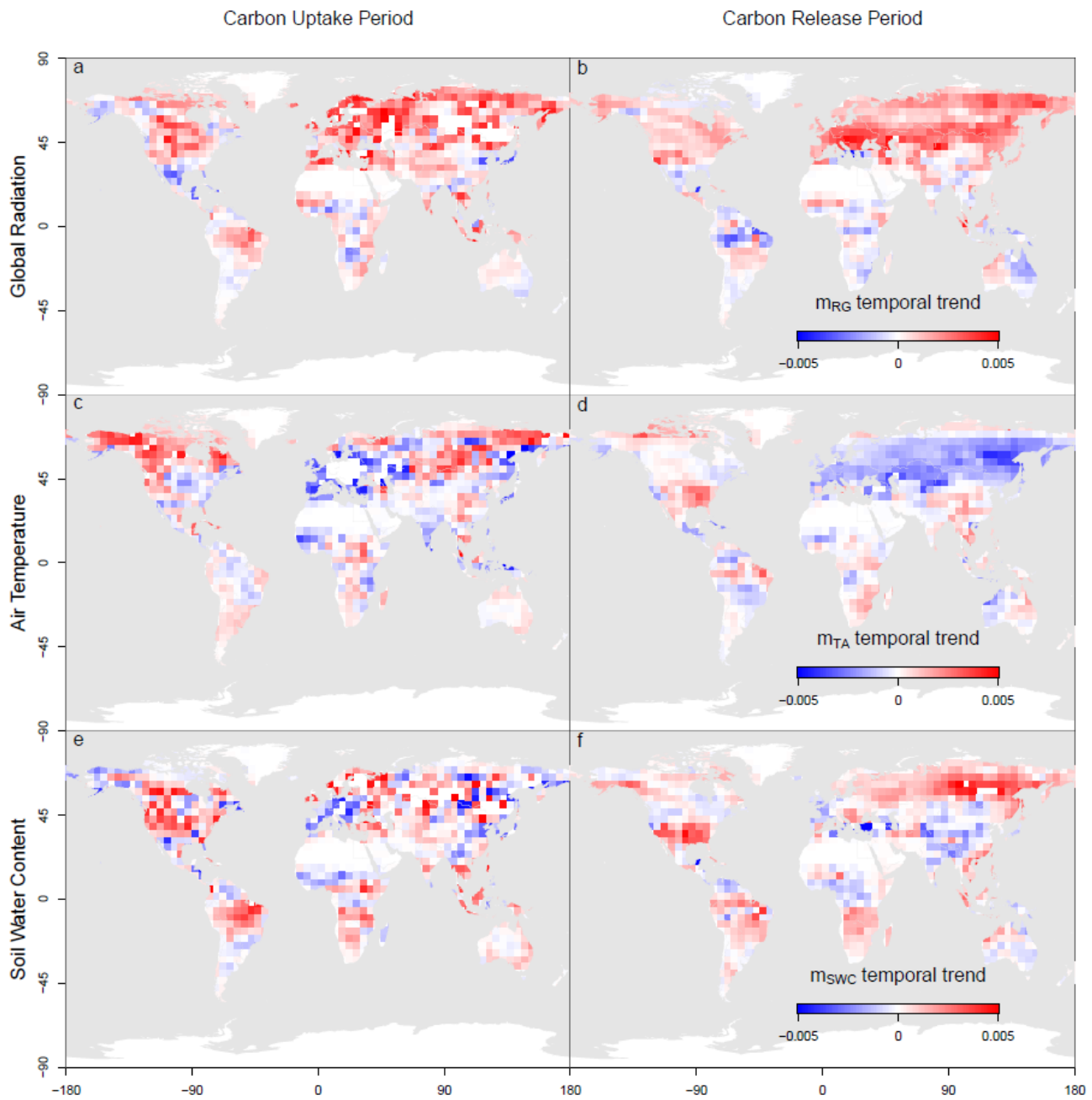
Figure 6 – Maps of sensitivity temporal trends separately shown for Carbon Uptake Period (CUP, left column) and Carbon Release Period (CRP, right column) at weekly time scale. Maps are plotted for global radiation (first row), air temperature (second row) and soil water content (third row).
