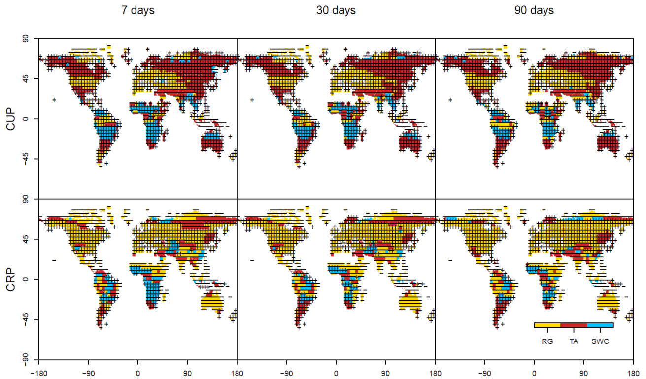
595 Figure 2 - Maps of the dominant drivers and sign of their angular coefficients in a multi-linear regression calculated separately for Carbon Uptake Period (CUP, top row) and Carbon Release Period (CRP, bottom row). Results are shown for three temporal resolutions, namely 7, 30 and 90 days.
