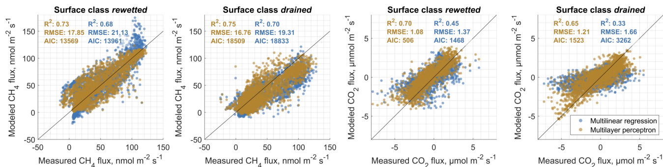
Figure 5. Comparative validation of surface class-specific multilinear regression and artificial neural network (in particular multilayer perceptron) carbon dioxide ( \text{CO}_2 ) and methane ( \text{CH}_4 ) flux models. For this depiction, we drove models that were optimized using Year 1 measurement data as targets with Year 2 environmental data and compared the results to measured Year 2 gas fluxes. This type of comparison enables an evaluation of the developed models with observed data which is completely independent from model optimization. Therefore, good agreement cannot be attributed to models which are overfit to the provided target data. The results of this investigation substantiate the notion that multilayer perceptrons provide more reliable estimates of gas fluxes as they are superior to multilinear models with respect to the coefficient of determination ( R^2 ), the Akaike information criterion (AIC) and the root mean squared error (RMSE) in all cases.
