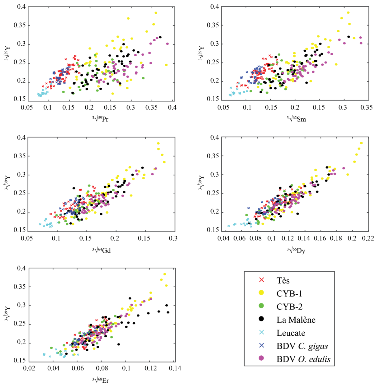
545 Figure 4: Gradual decrease of REE abundances in oyster shells according to the REE atomic number, presented against Y. Values are expressed in cubic root of abundances (in \mu\text{g.g}^{-1} ) to approach normality. Measurements from C. gigas and O. edulis are indicated with crosses and filled circles, respectively.
