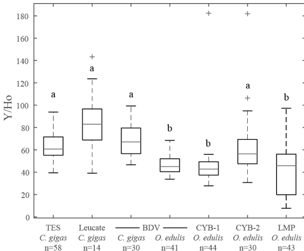
540 Figure 3: Boxplots of Y/Ho ratios for all groups. The letters on top of the boxes (a and b) identify the significant differences between groups from Kruskal-Wallis tests. Note that for the same locality at Baie des Veys, the Y/Ho ratios are significantly different depending on the species considered (BDV C. gigas and O. edulis groups). Grey bars represent median values, the lower and higher large black bars represent the 25 th and 75 th percentiles, respectively, and the lower and higher small black bars represent the minimum and maximum values not considered as outliers, respectively. Outliers are represented by grey crosses.
