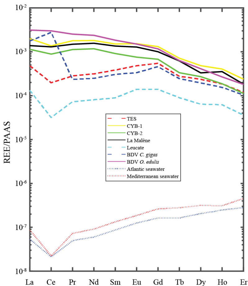
550 Figure 5: REE median profiles for all groups of oyster specimens. Crassostrea gigas groups are symbolized with dashed lines and continuous lines for O. edulis groups. Seawater profiles of the Atlantic Ocean (van der Flierdt et al., 2012) and the Mediterranean Sea (Censi et al., 2004) are indicated for comparison. Values are normalized to Post-Archean Australian Shales (PAAS) according to McLennan (1989).
