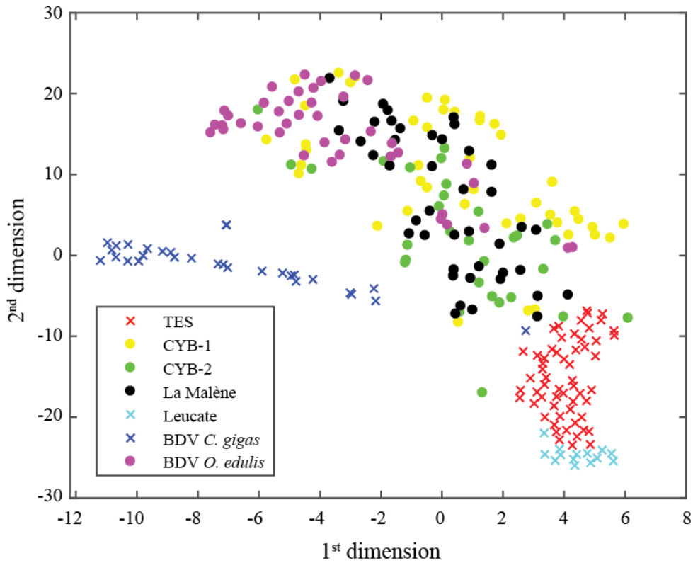
Figure 6: Visualization of shell group partitioning using t-SNE applied to all REE and Y measurements as variables. Crosses and large dots refer to C. gigas and O. edulis , respectively.
