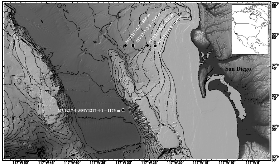
915 Figure 1. Map of cores used in this study. The cores were collected along a transect perpendicular to shore at the following water depths: 300, 528, 700, 800, 1175 m. Core top samples were analyzed for all cores. Cores MV1217-2-3, MV1217-1-3, and MV1217-4-3/MV1217-4-1 were analyzed down core.
