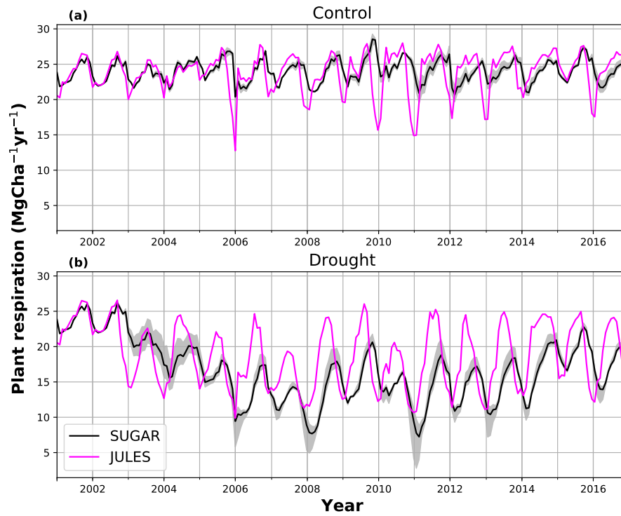
Figure A4. Simulated plant respiration ( R ) from JULES and SUGAR for (a) the control and (b) the through-fall exclusion (TFE) plots at Caxiuanã. A sensitivity study on the parameter a_{K_m} in SUGAR was carried out and the maximum, minimum and ensemble mean R are presented. Time-series observations of R from the site were not available.
